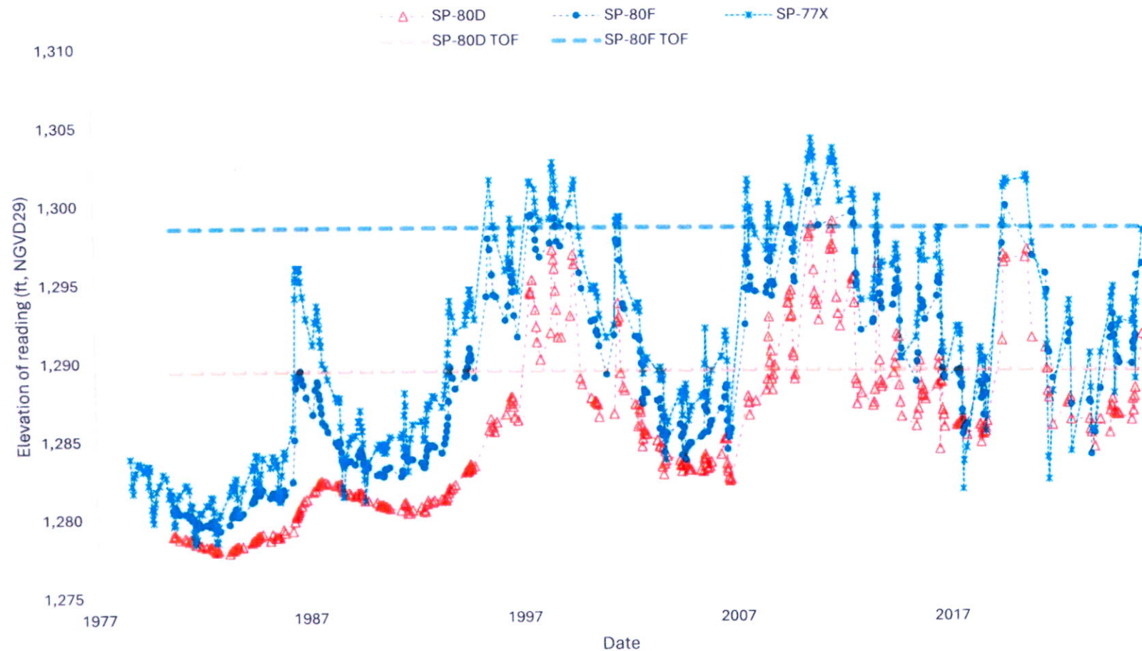
Observation Well Water Elevations Near App. Nos. 9002-3 and 9003-3
