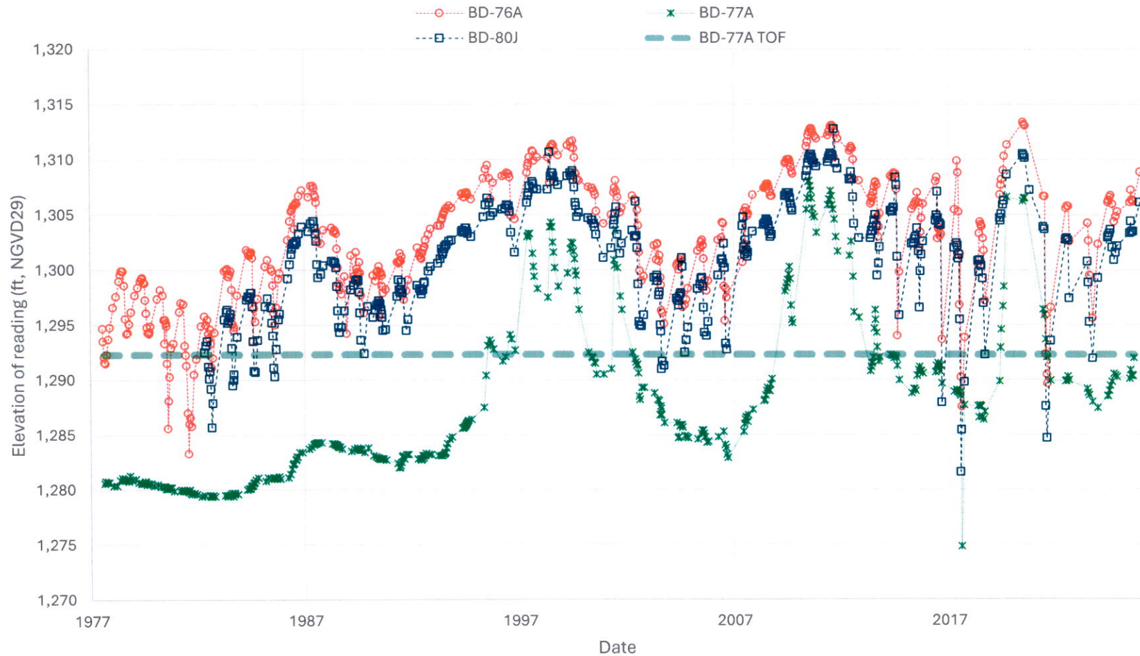
Observation Well Water Elevations Near App. Nos. 9001-3 and 9004-3
