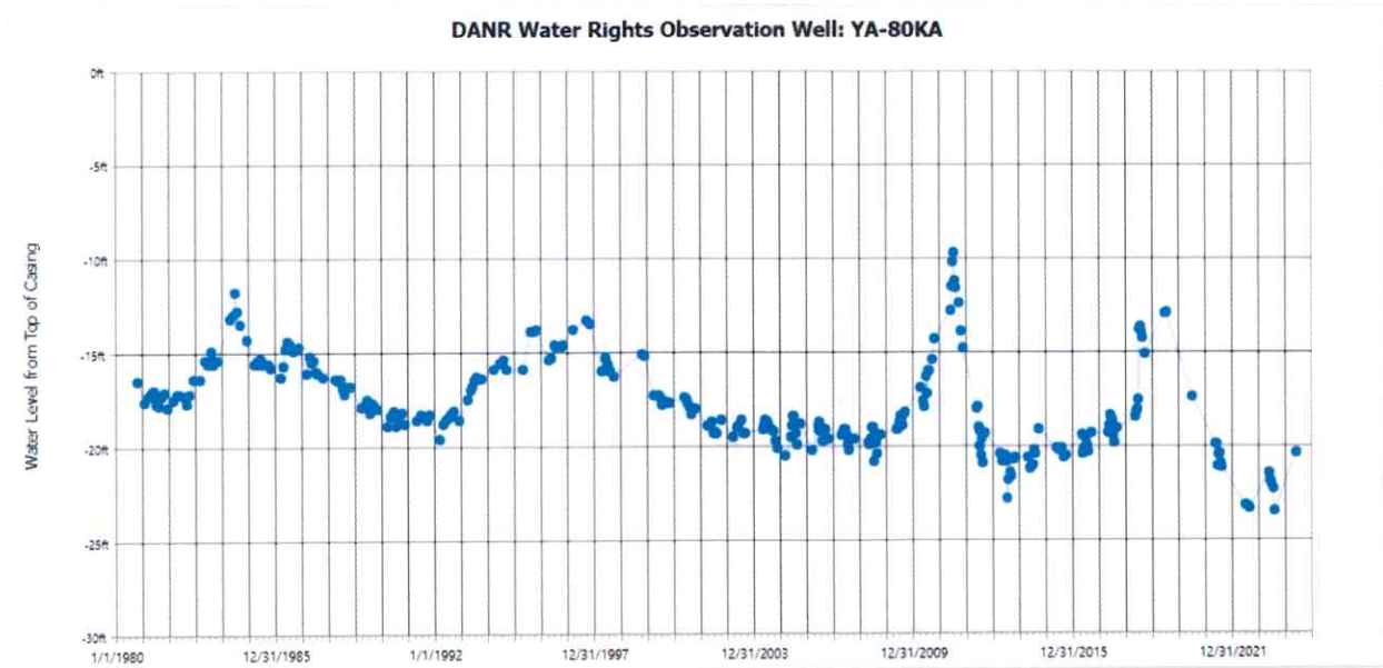
Figure 2. Hydrograph for observation well YA-80KA (Water Rights, 2024b)
