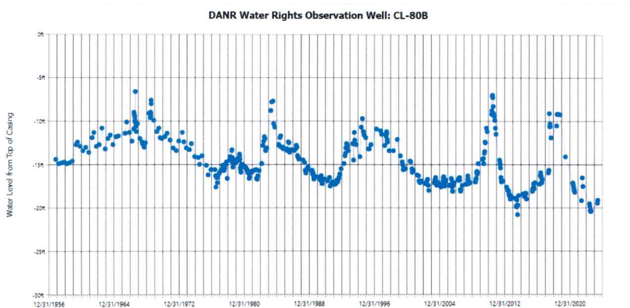
Figure 4. Hydrograph for observation well CL-80B (Water Rights, 2024b)
