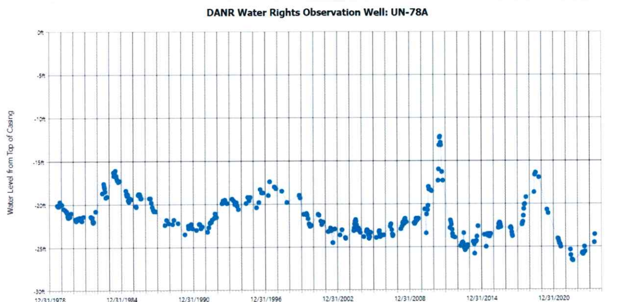
Figure 4. Hydrograph for observation well UN-78A (Water Rights, 2024b)
