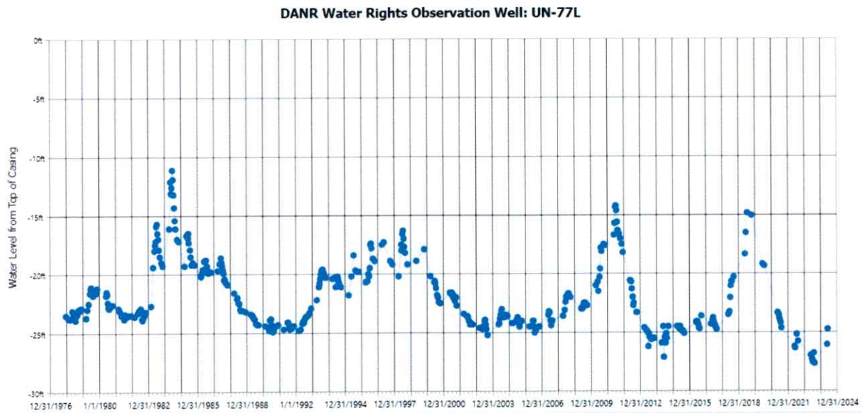
Figure 2. Hydrograph for observation well UN-77L (Water Rights, 2024b)
