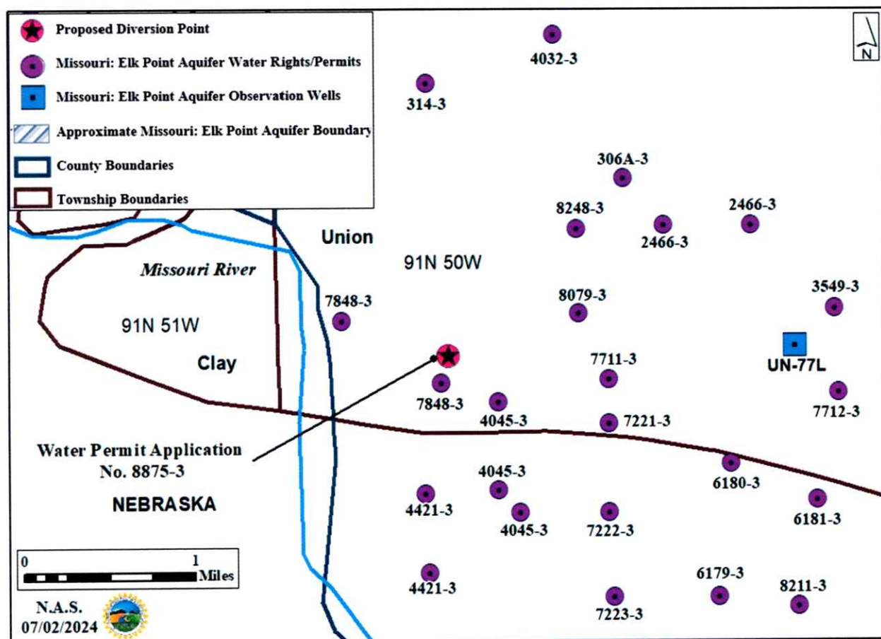
Figure 6. Location of the proposed diversion point for Water Permit Application No. 8875-3 and the Missouri: Elk Point aquifer water rights/permits and observation well within approximately two miles (Water Rights, 2024b and 2024c)
