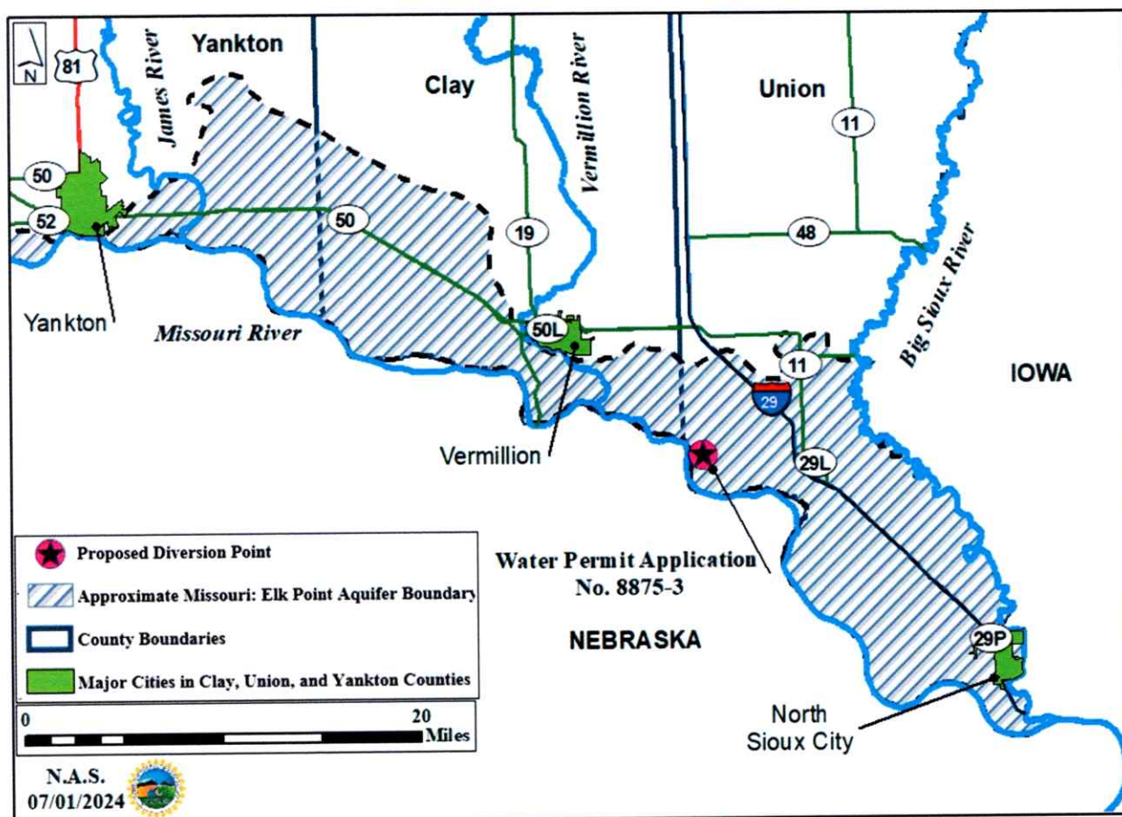
Figure 1. Map of the approximate Missouri: Elk Point aquifer boundary modified from Hedges and others (1982) with the location of the proposed diversion point for Water Permit Application No. 8875-3 (Water Rights, 2024c and 2024d)
