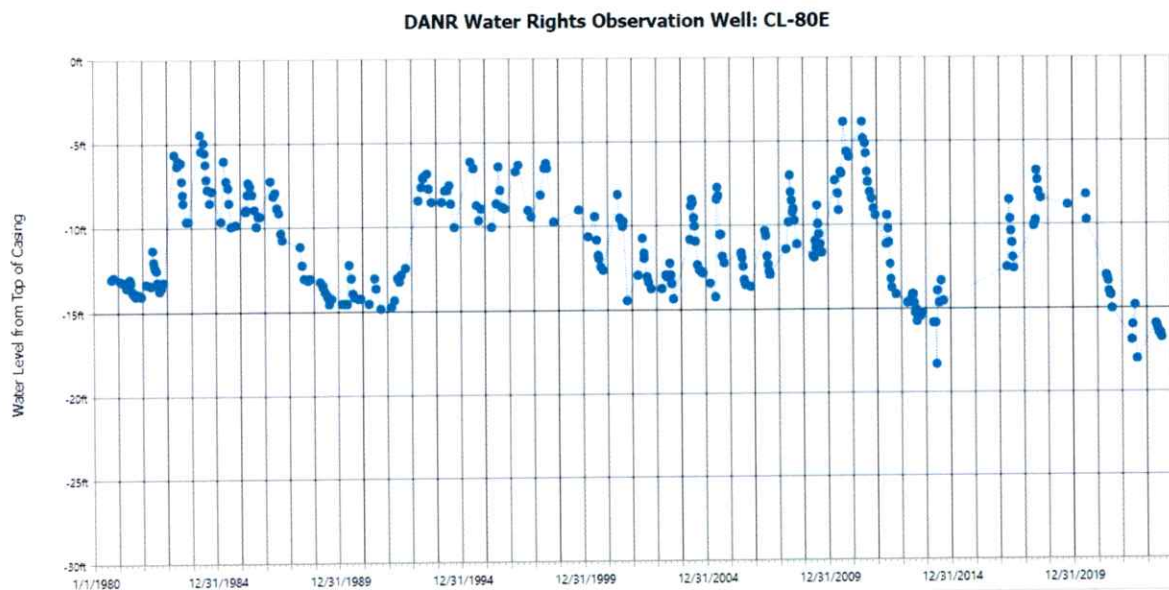
Figure 3. Hydrograph for observation well CL-80E (Water Rights, 2024b)
