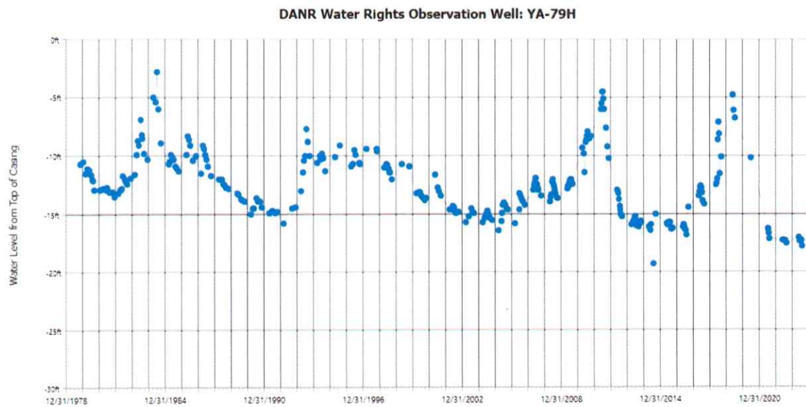
Figure 4. Hydrograph for observation well YA-79H (Water Rights, 2024b)
