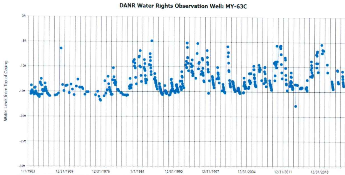
Figure 3. Hydrograph for observation well MY-63C (Water Rights, 2023b)
