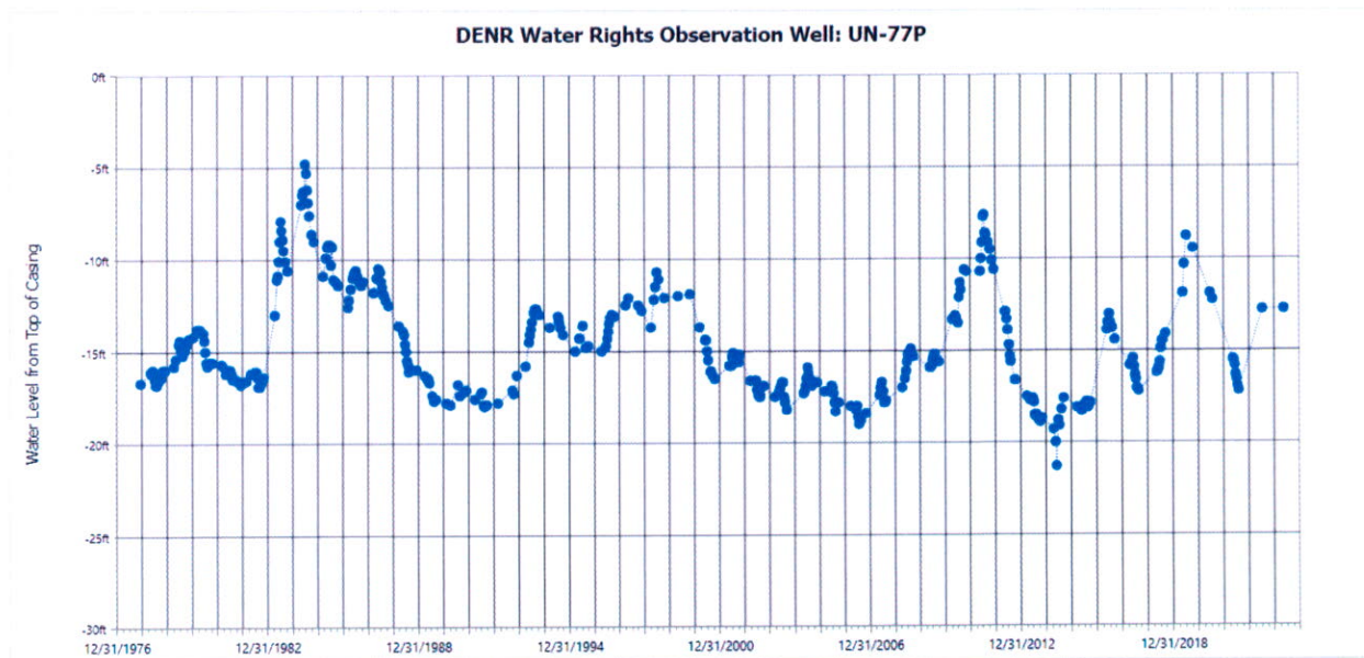
Figure 4. Hydrograph for observation well UN-77P (Water Rights, 2023b)
