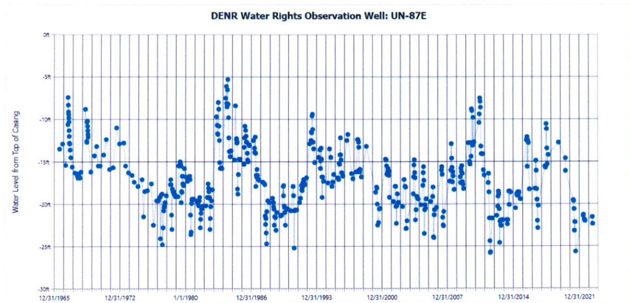
Figure 3. Hydrograph for observation well UN-87E (Water Rights, 2023b)
