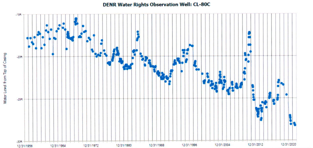
Figure 4. Hydrograph for observation well CL-80C (Water Rights, 2023b)
