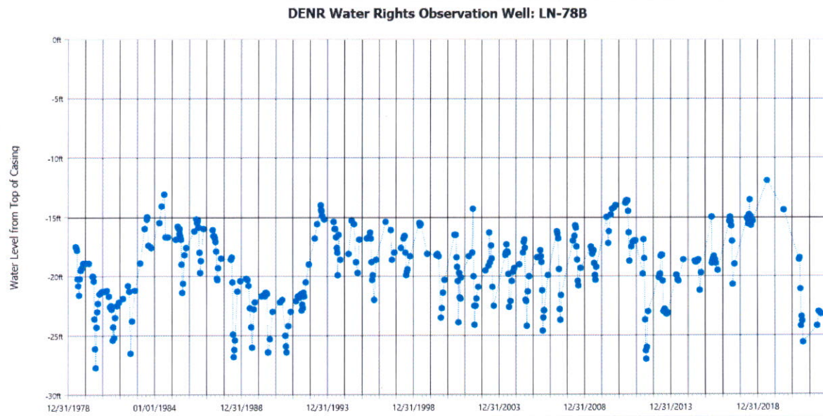
Figure 4. Hydrograph for observation well LN-78B (Water Rights, 2023a)
