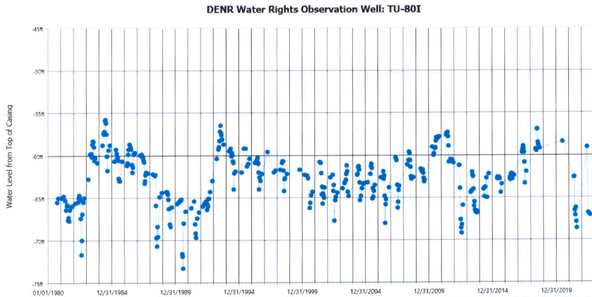
Figure 3. Hydrograph for observation well TU-80I (Water Rights, 2023a)
