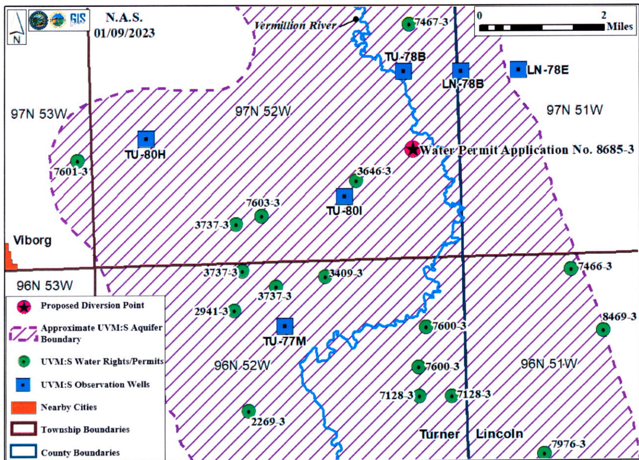
Figure 6. Location of the proposed diversion point for Water Permit Application No. 8685-3 with the Upper Vermillion Missouri: South aquifer water rights/permits and observation wells within approximately five miles (Water Rights, 2023a and 2023b)
