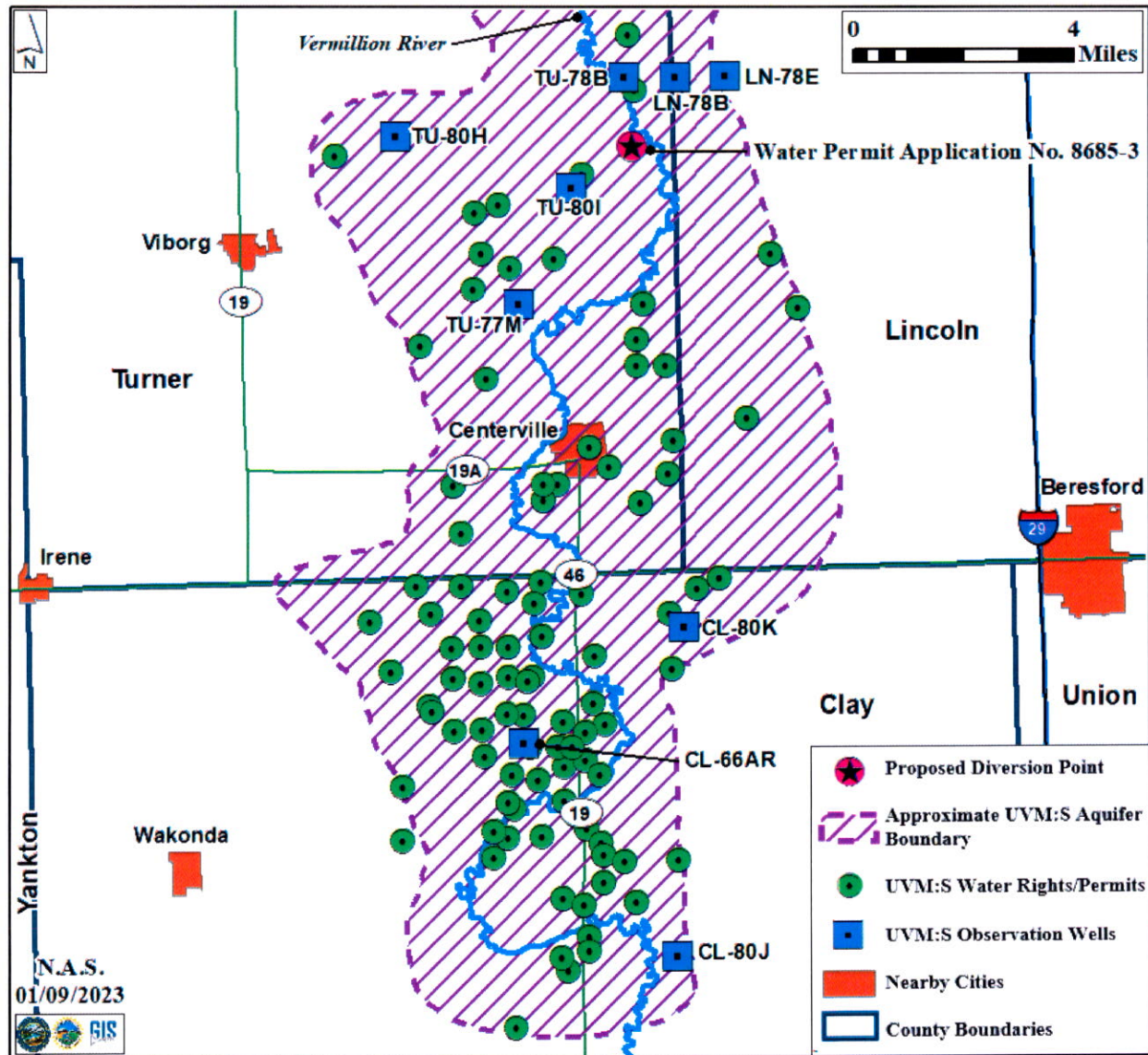
Figure 1. Map of the approximate Upper Vermillion Missouri: South aquifer delineated from Buhler (2014), the location of the proposed diversion point for Water Permit Application No. 8685-3, and the Upper Vermillion Missouri: South aquifer water rights/permits and observation wells (Water Rights, 2023a and 2023b)
