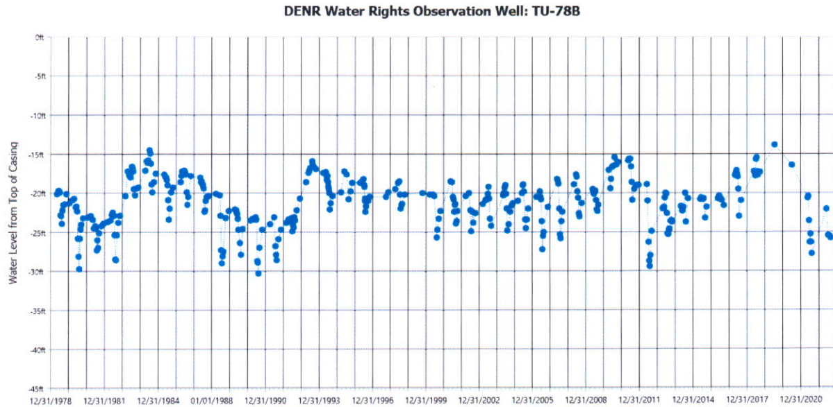
Figure 2. Hydrograph for observation well TU-78B (Water Rights, 2023a)
