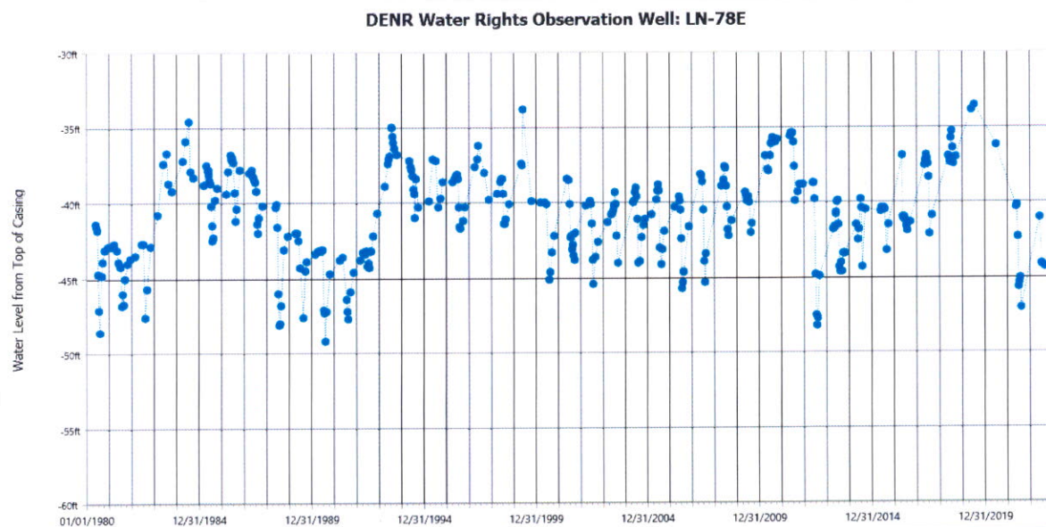
Figure 5. Hydrograph for observation well LN-78E (Water Rights, 2023a)
