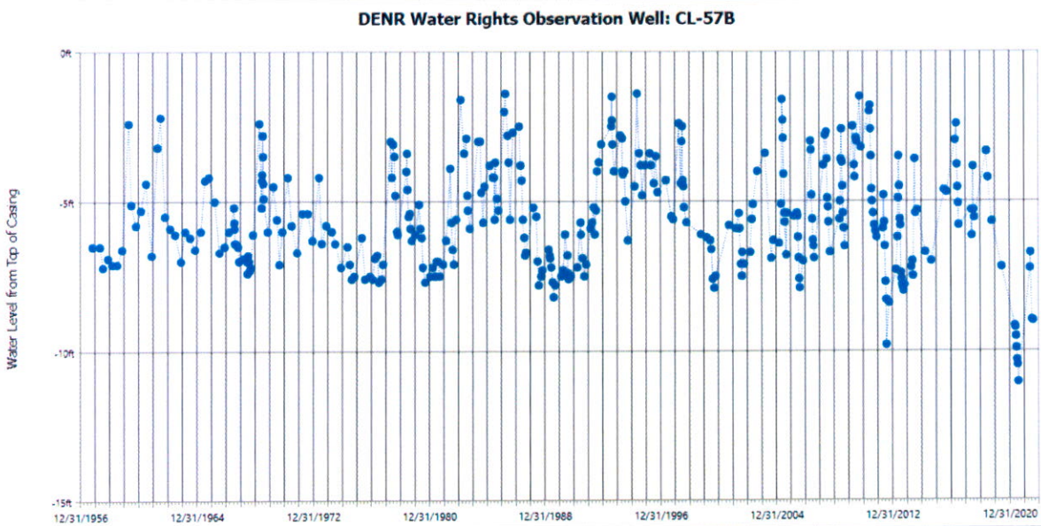
Figure 3. Hydrograph for observation well CL-57B (Water Rights, 2023b)
