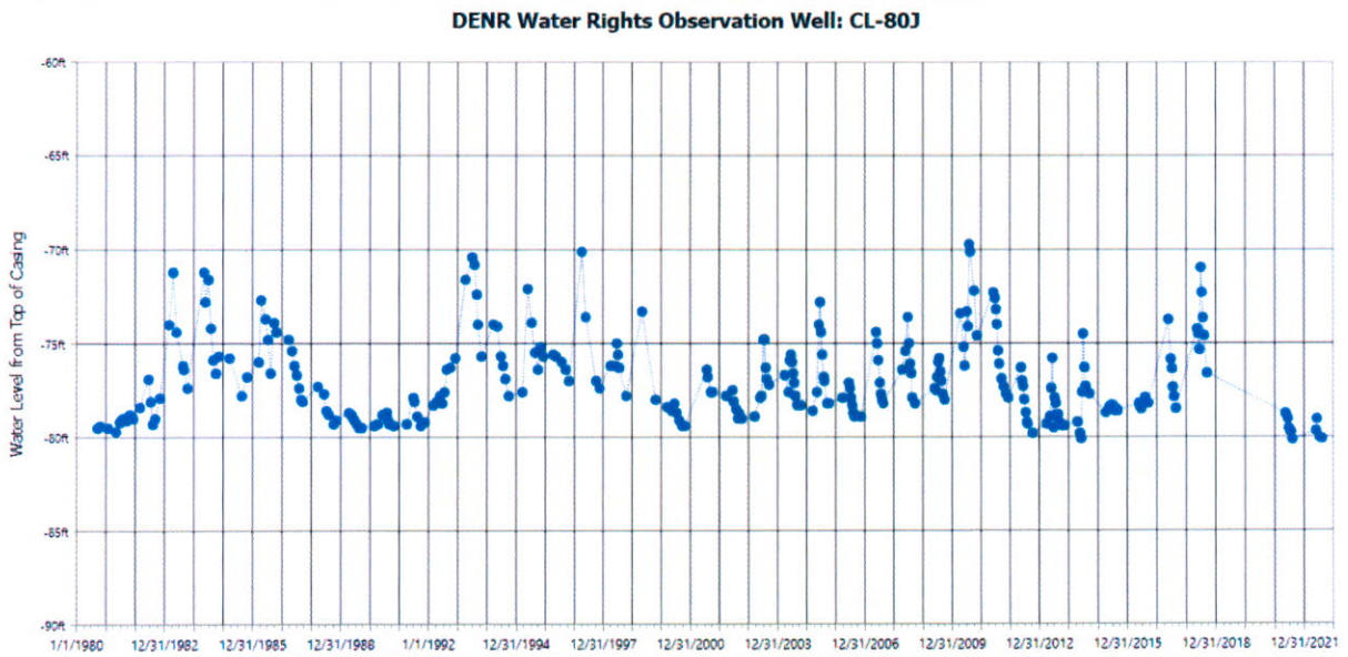
Figure 2. Hydrograph for observation well CL-80J (Water Rights, 2023b)
