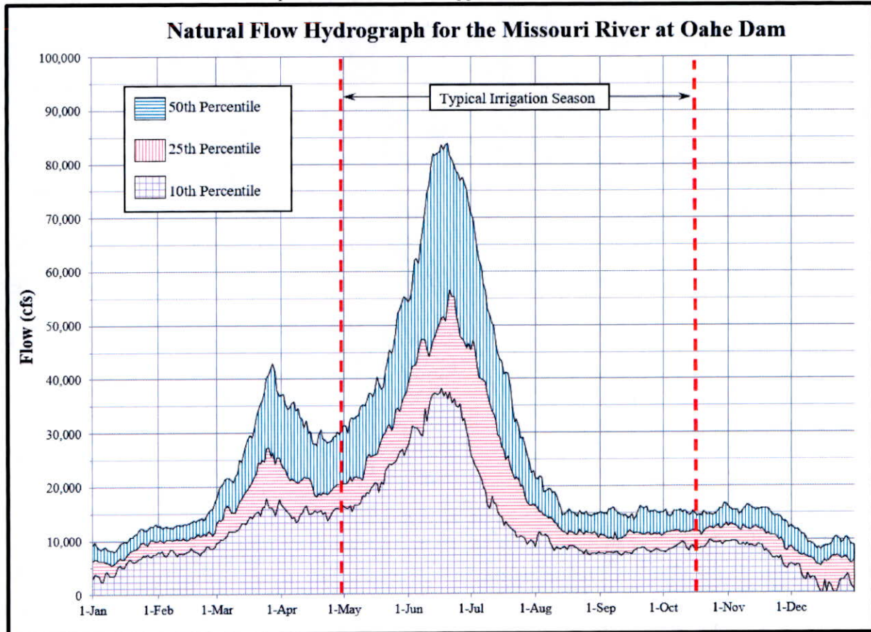
Figure 1. Natural Flow Hydrograph for the Missouri River at Oahe Dam (Jacobson, 2001).
