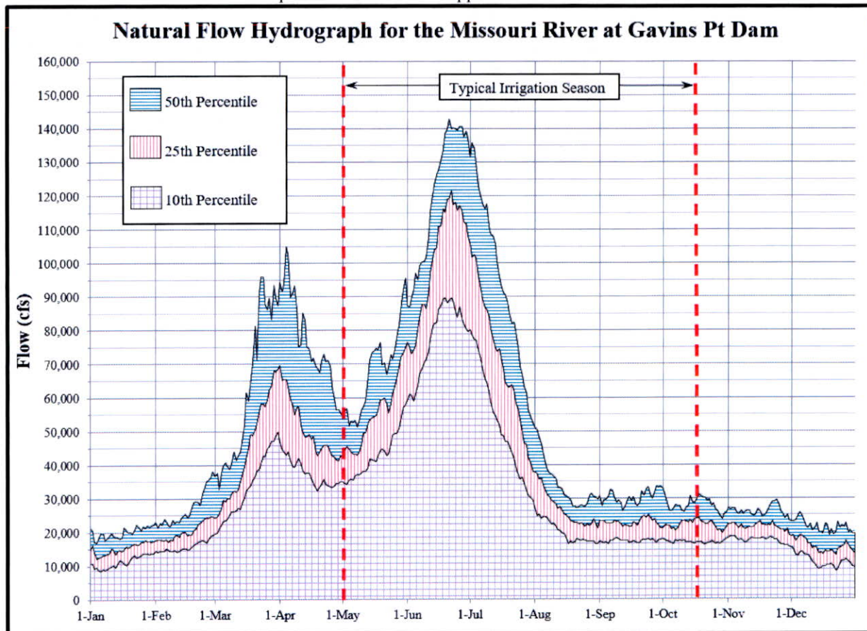
Figure 2. Natural Flow Hydrograph for the Missouri River at Gavins Point Dam (Jacobson, 2001).
