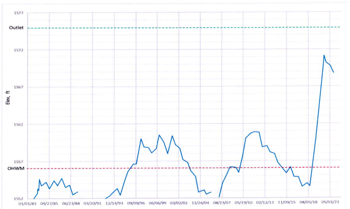
Figure 1. Lake level hydrograph for Red Lake in Brule County South Dakota, 1983-2021 (Water Rights. 2022).
