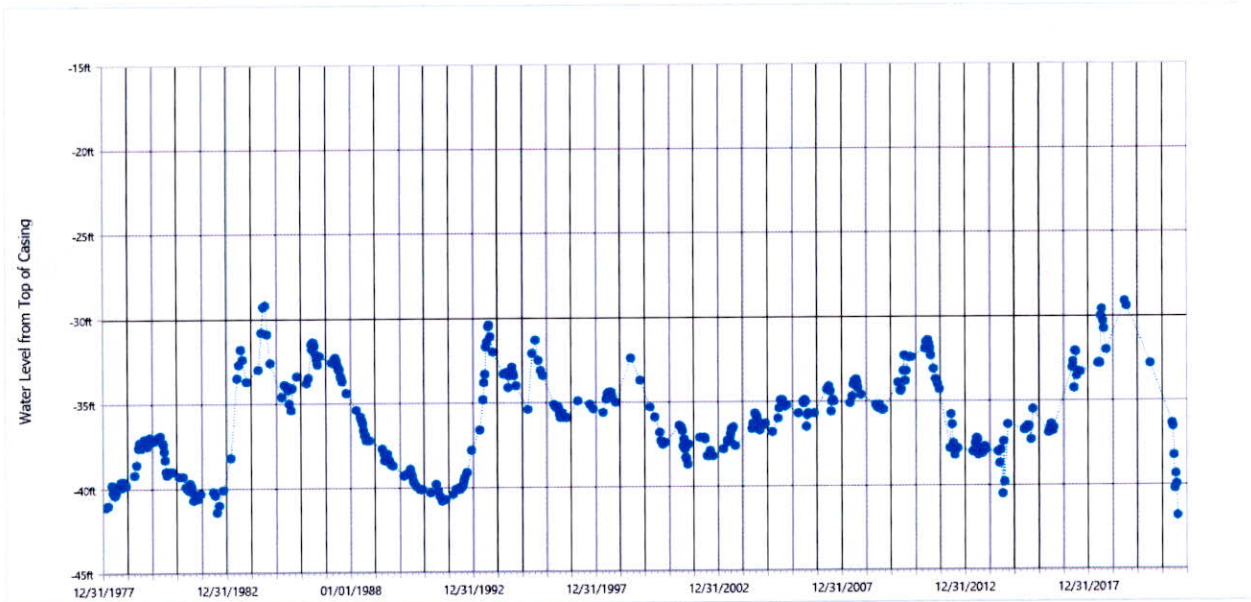
Figure 2: Hydrograph of the Upper Vermillion Missouri: West aquifer observation well TU-77T, located approximately one mile northwest of the proposed diversion point (Water Rights, 2022b).
