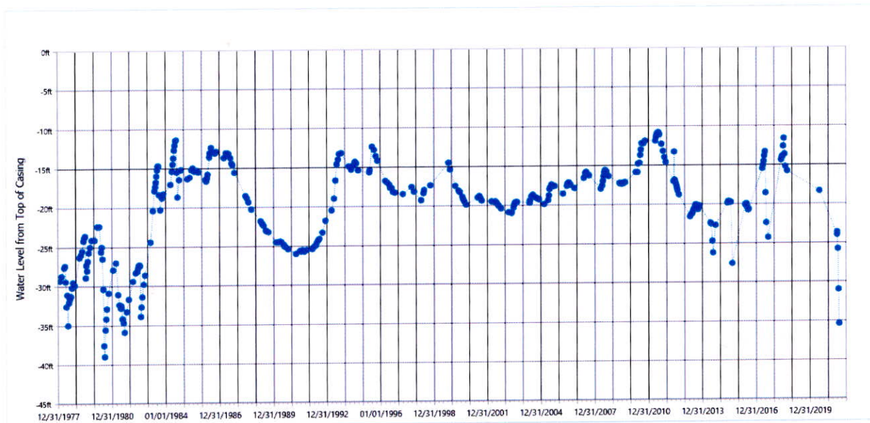
Figure 3: Hydrograph of the Upper Vermillion Missouri: West aquifer observation well TU-77S, located approximately 8.1 miles northwest of the proposed diversion point (Water Rights, 2022b).
