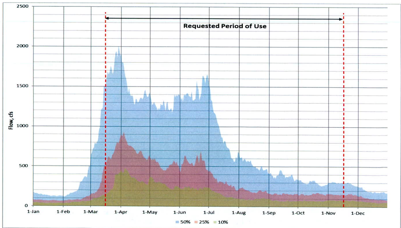
Figure 1. Daily percentile flow hydrographs for the USGS 06485500 Big Sioux River gage at Akron IA 1928-2021, contributing drainage area 6,995 mi 2 (USGS, 2021).
