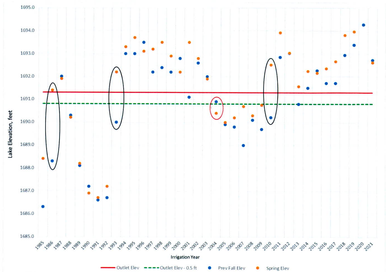
Figure1. Lake Alice lake level hydrograph with the lake outlet elevation and proposed irrigation trigger elevation based upon 37 years of record, (Water Rights. 2021).
