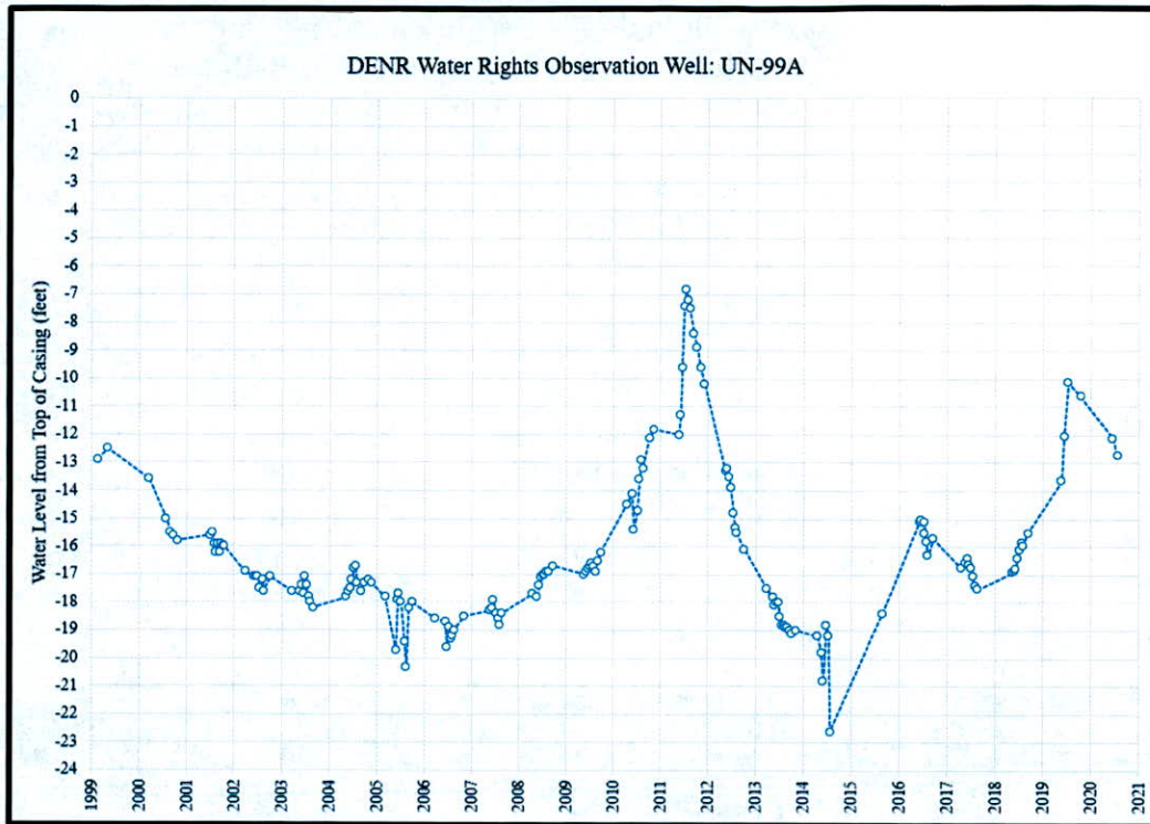
Figure 4. Hydrograph for observation well UN-99A located approximately 1.7 miles south of the proposed well location for Water Permit Application No. 8489-3 (Water Rights, 2021c).
