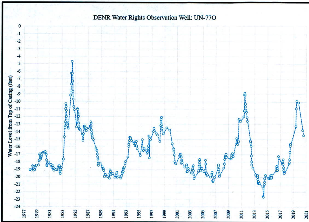
Figure 2. Hydrograph for observation well UN-77O located approximately 3.6 miles north of the proposed well location for Water Permit Application No. 8489-3 (Water Rights, 2021c).
