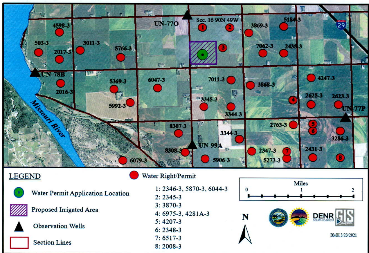
Figure 7. Existing Missouri: Elk Point aquifer water rights/permits and observation wells in the vicinity of Water Permit Application No. 8489-3 (modified from Hedges, et al., 1982; Water Rights 2021a & 2021c).
