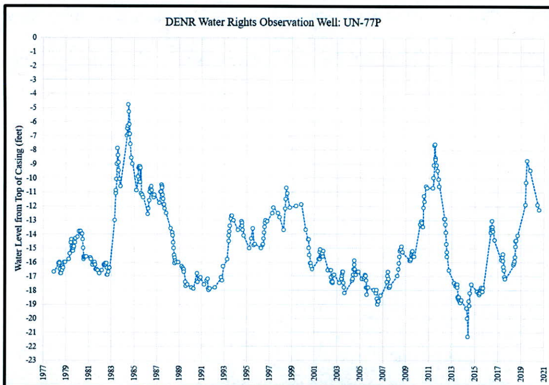
Figure 3. Hydrograph for observation well UN-77P located approximately 2.9 miles southeast of the proposed well location for Water Permit Application No. 8489-3 (Water Rights, 2021c).
