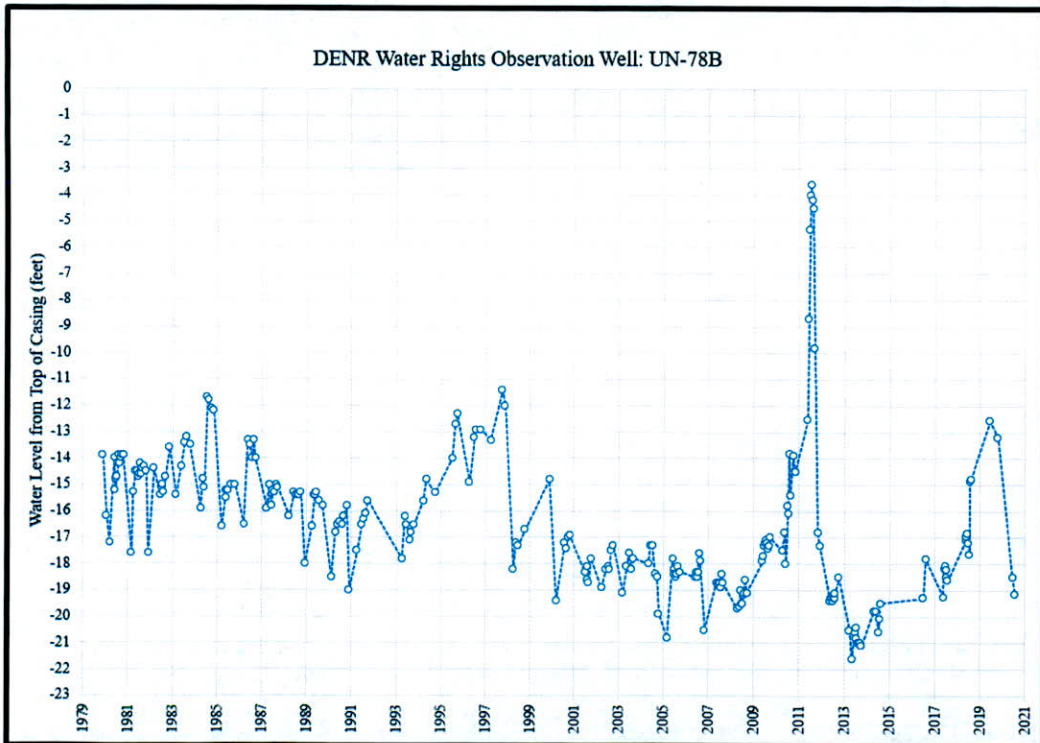
Figure 5. Hydrograph for observation well UN-78B located approximately 3.1 miles west of the proposed well location for Water Permit Application No. 8489-3 (Water Rights, 2021c).
