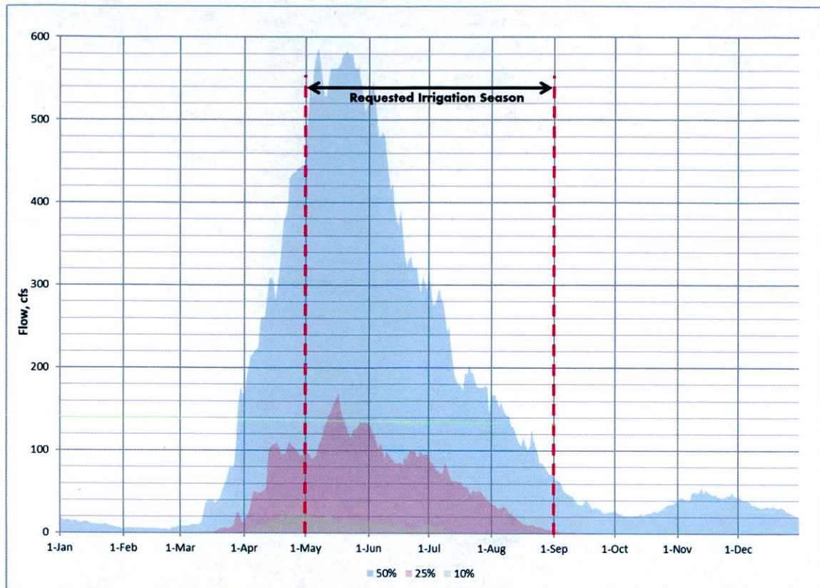
Figure 2. Daily percentile flow hydrograph for the USGS gaging station No. 06473000, 1945-2020, on the James River at Ashton, SD, contributing drainage area 8,333 mi 2 , (USGS, 2021).
