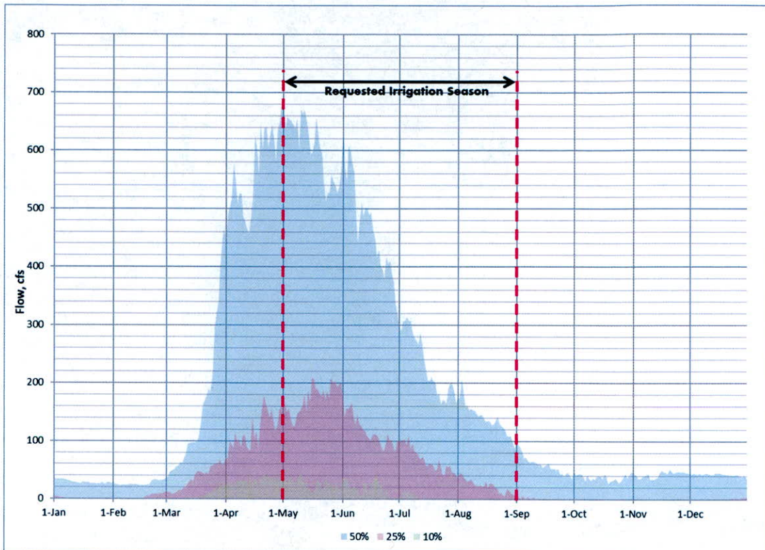
Figure 3. Daily percentile flow hydrograph for the USGS gaging station No. 06476000, 1943-2020, on the James River at Huron, SD, contributing drainage area 13,795 mi 2 , (USGS, 2021).
