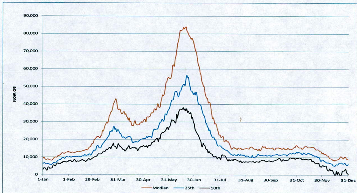
Figure 1. Natural Flow Hydrograph for the Missouri River at Oahe Dam (Jacobson, 2001).
