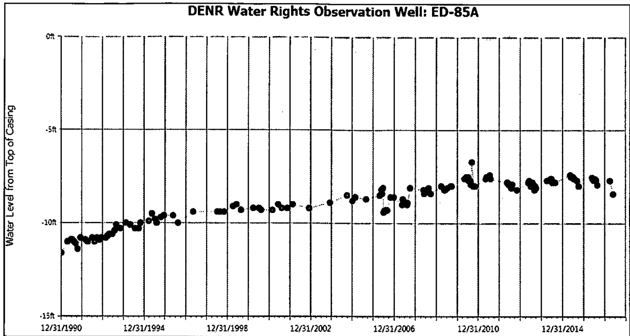
Figure 2: Hydrograph for Observation Well ED-85A (Water Rights, 2018c)
