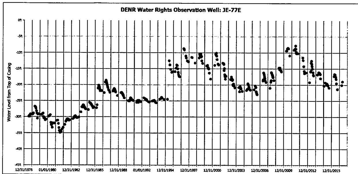
Figure 1. Hydrograph of observation well JE-77E.
