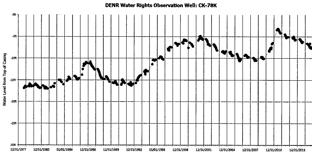
Figure 3: Hydrograph for Observation Well CK-78K located approximately four miles to the south southeast of the proposed well location for this application (Water Rights, 2016a)
