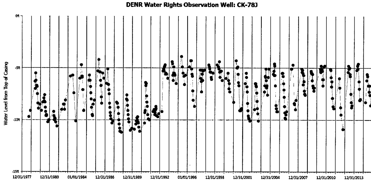
Figure 2: Hydrograph for Observation Well CK-78J (Water Rights, 2016a)
