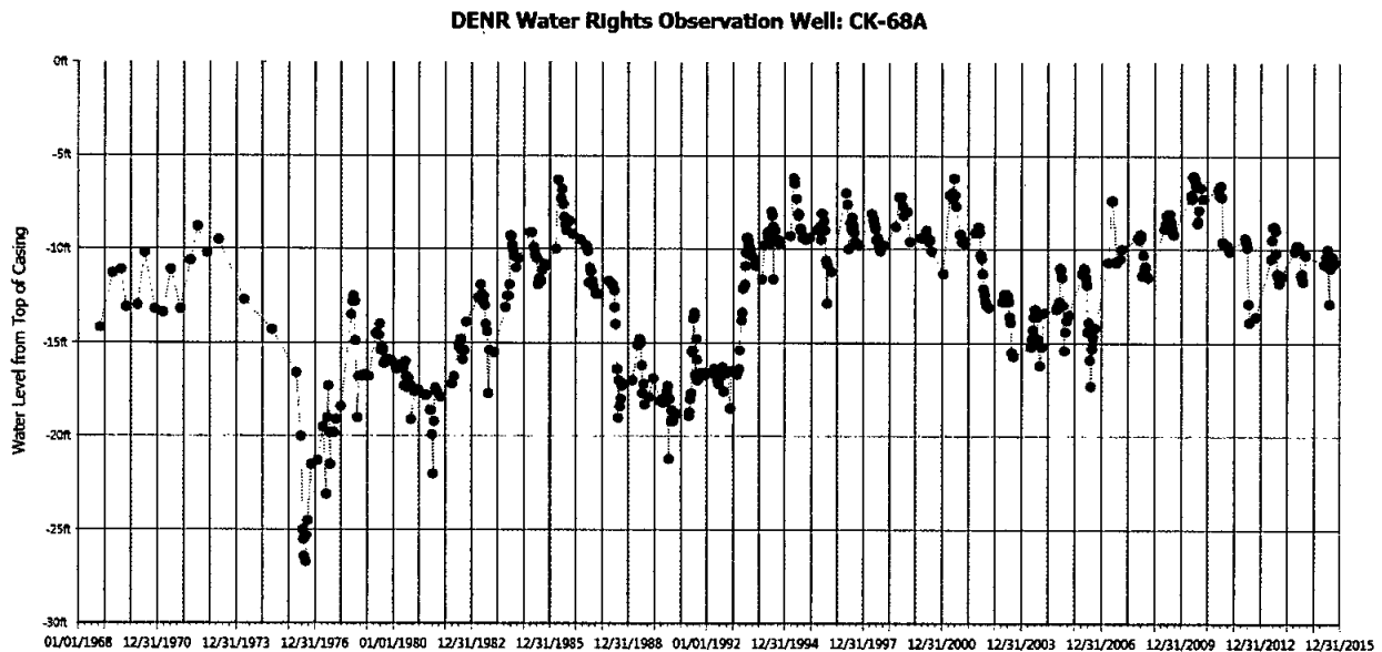
Figure 5: Hydrograph for Observation Well CK-68A located approximately 7.4 miles to the south southeast of the proposed well location for this application (Water Rights, 2016a)
