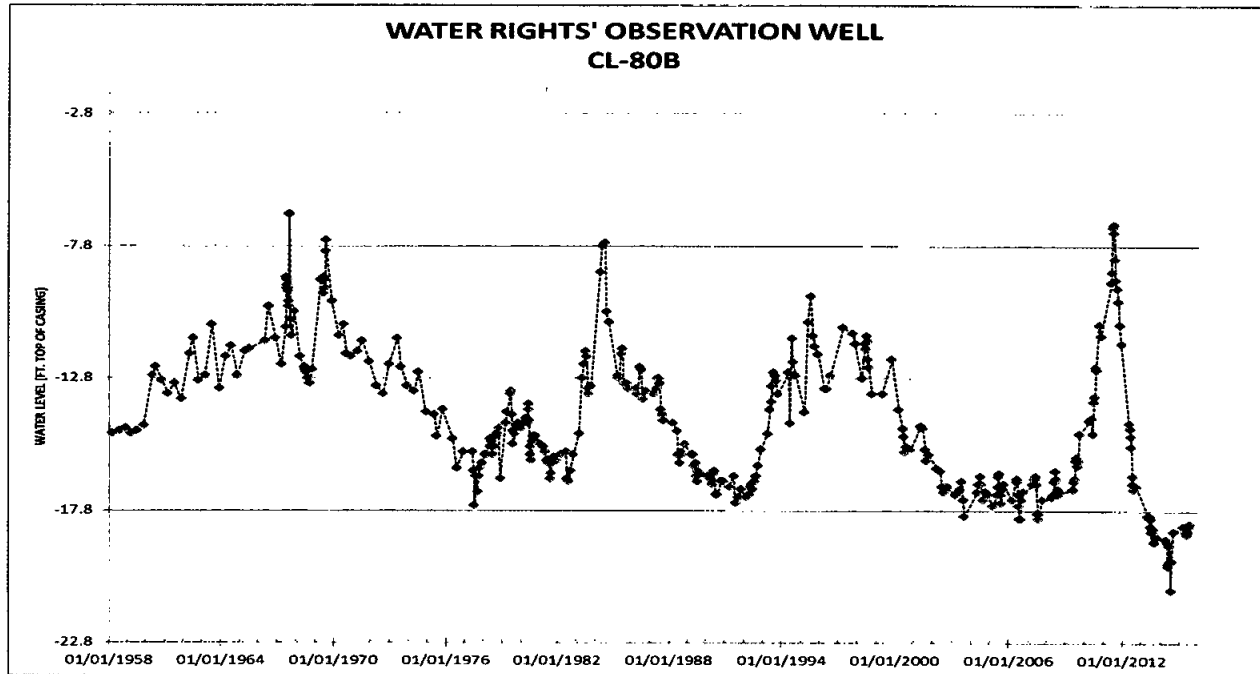
Figure 1. Hydrograph of DENR-Water Rights' Observation Well CL-80B which is completed into the Missouri Elk Point aquifer.
