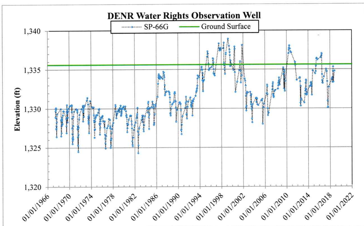
Figure 4. Hydrograph of DENR-Water Rights' observation well SP-66G (see Figure 1 for location). Top of aquifer elevation is approximately 1264 ft.
