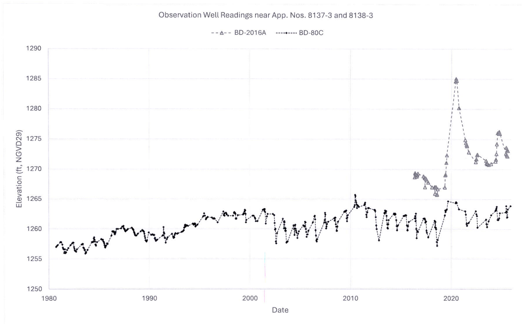
Figure 2: Observation well readings near these applications [2]
