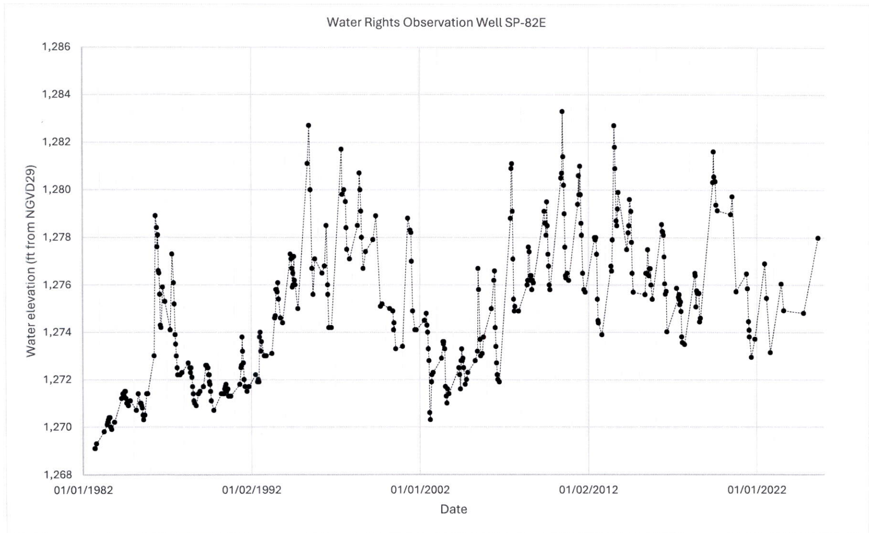
Figure 2: Hydrograph of Observation Well SP-82E [2]
