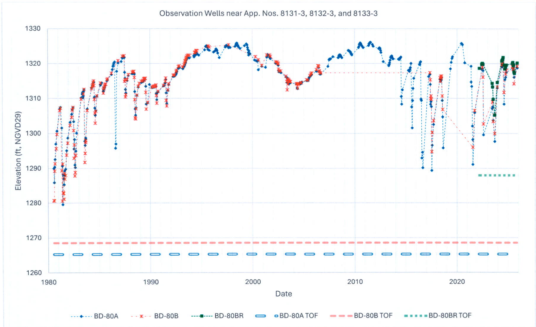
Figure 2: Observation water elevations near App. Nos. 8131-3, 8132-3, and 8133-3. TOF – Top of Formation [2]
