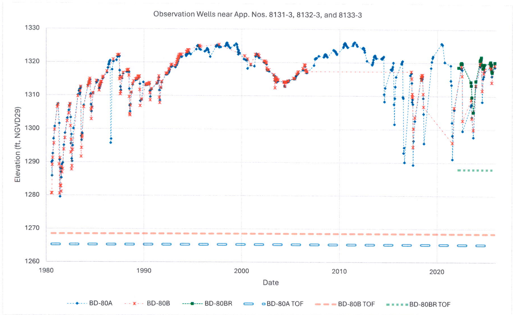
Figure 3: Observation water elevations near App. Nos. 8131-3, 8132-3, and 8133-3. TOF – Top of Formation [2]
