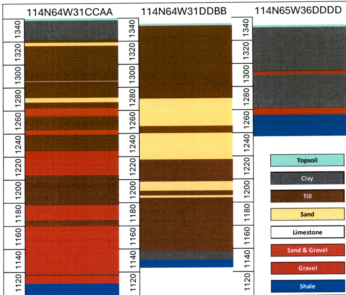
Figure 2: Lithologic logs near these applications [3]. The vertical scale is elevation in feet from NGVD29.
