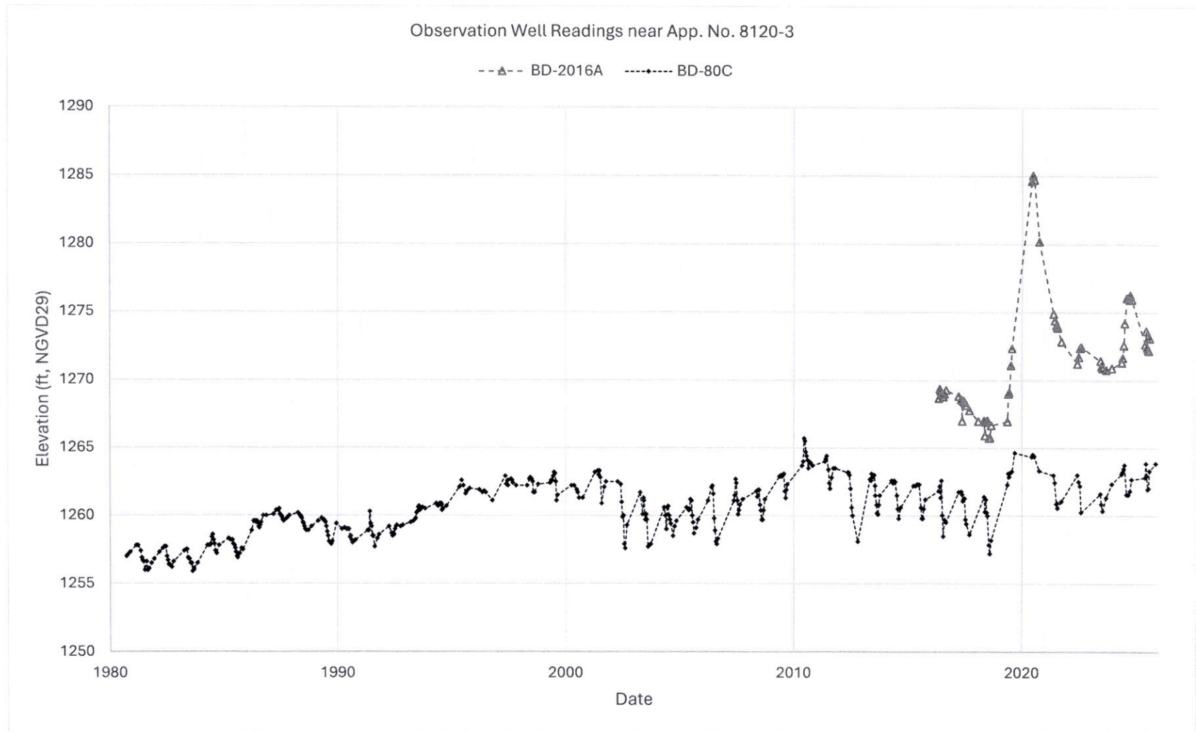
Figure 2: Observation well readings near this application [2]
