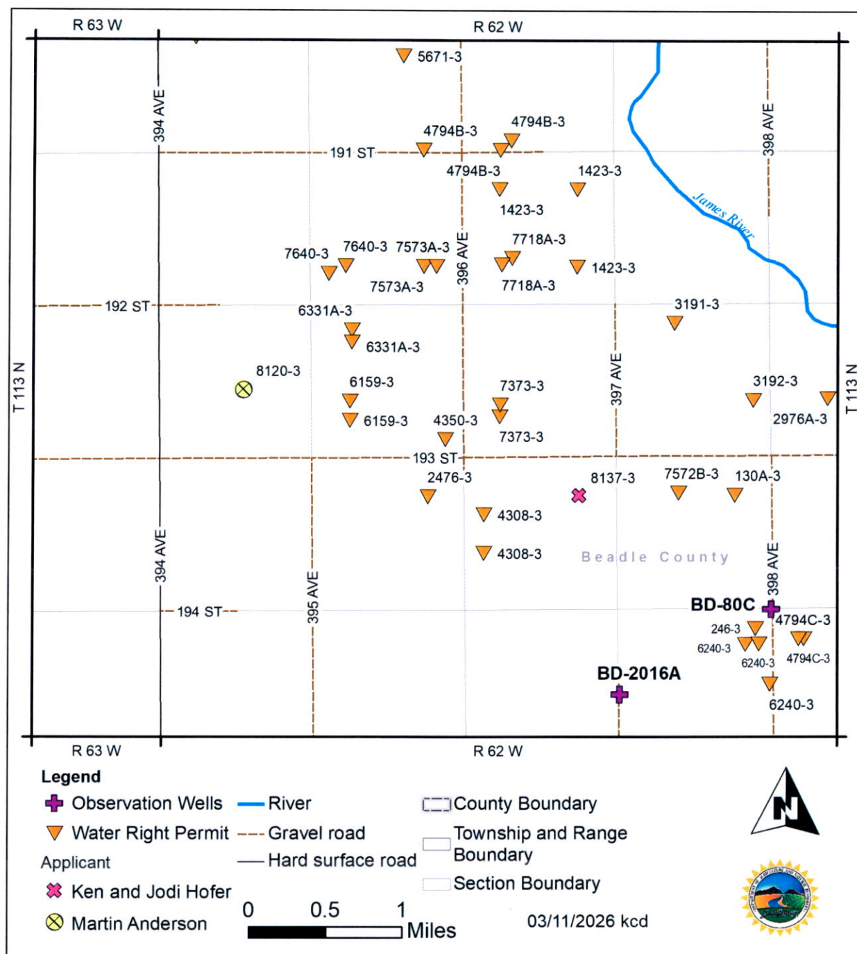
Figure 1: Observation wells, held applications, and water right permits near this application. [1] [2]
