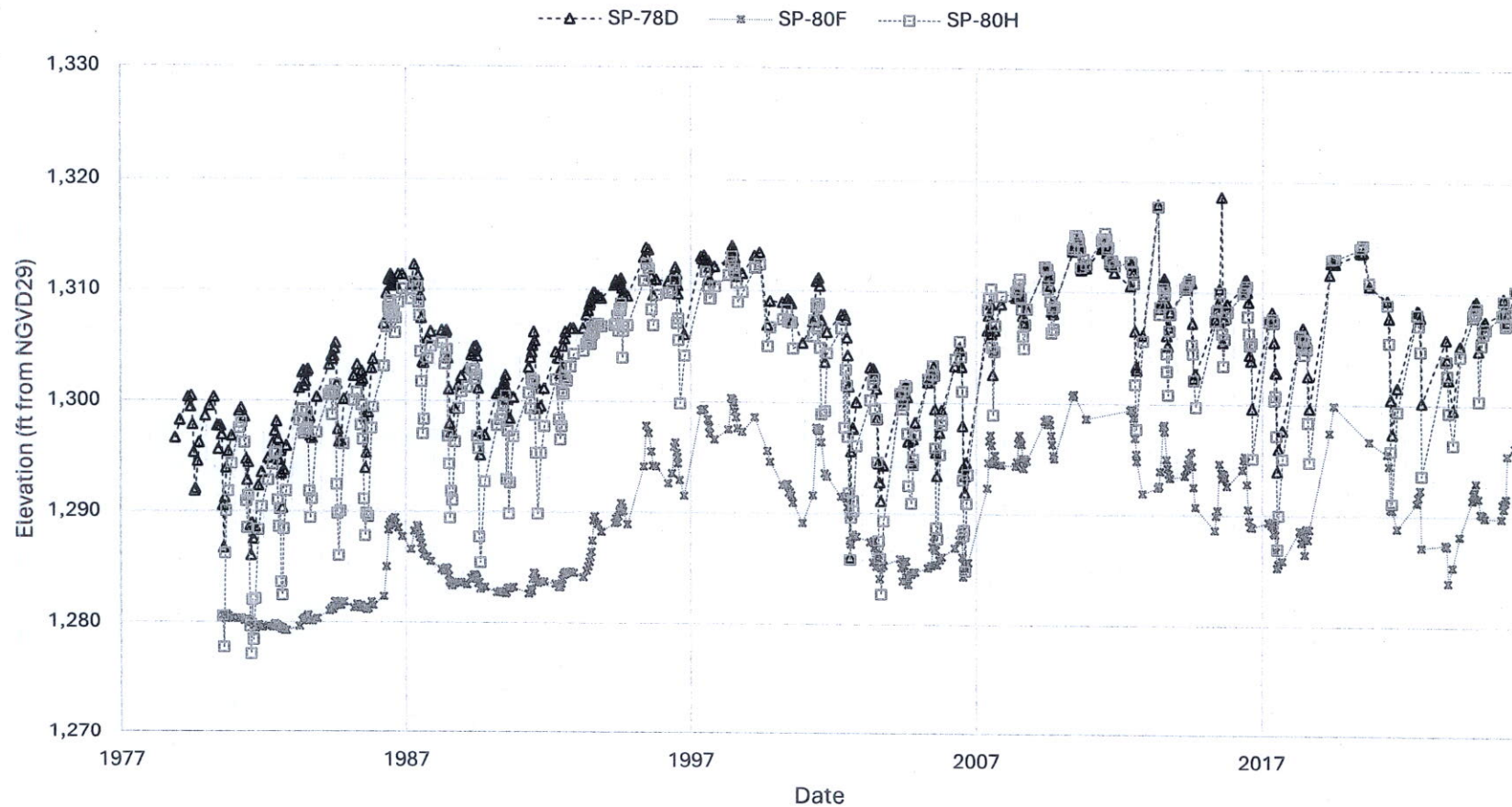
Figure 2: Observation well hydrographs for the observation wells near the northern edge of Figure 1 [2]
