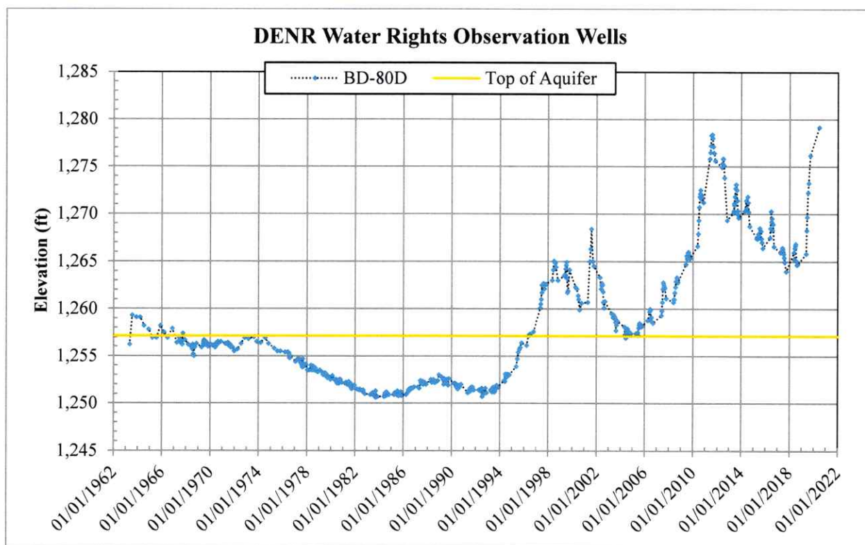
Figure 2. Hydrograph of DENR-Water Rights' observation well BD-80D (see Figure 1 for location). Ground surface elevation is approximately 1292 ft.
