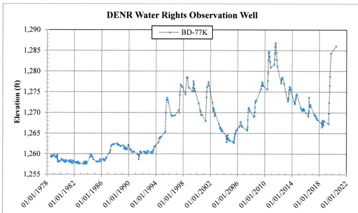
Figure 3. Hydrograph of DENR-Water Rights' observation well BD-77K (see Figure 1 for location). Top of aquifer elevation is approximately 1239 ft, ground surface elevation is approximately 1313 ft.
