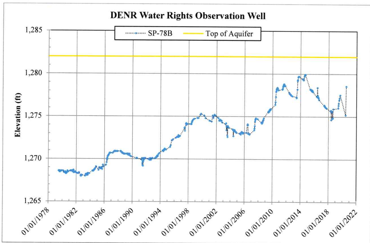
Figure 6. Hydrograph of DENR-Water Rights' observation well SP-78B (see Figure 1 for location). Ground surface elevation is approximately 1296 ft.
