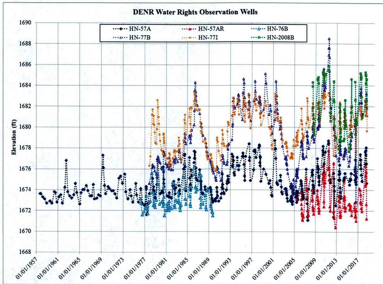
Figure 2: Hydrographs for Observation Wells HN-57A, HN-57AR, HN-76B, HN-77B, HN-77I, and HN-2008B. (Water Rights, 2018b)
