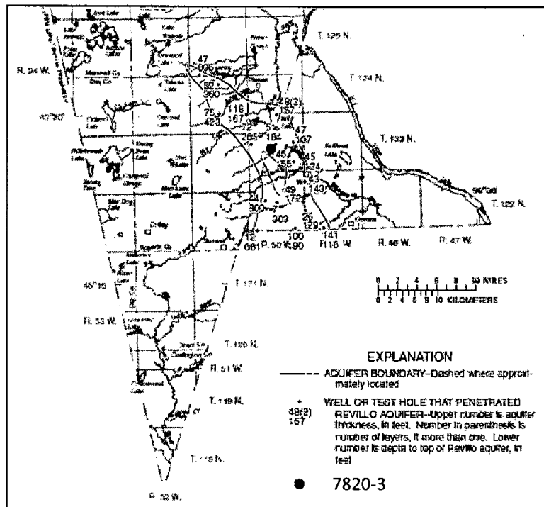
Figure 1- Thickness, depth, and extent of the Renvo aquifer in Roberts County (modified from Thompson, 2001)
