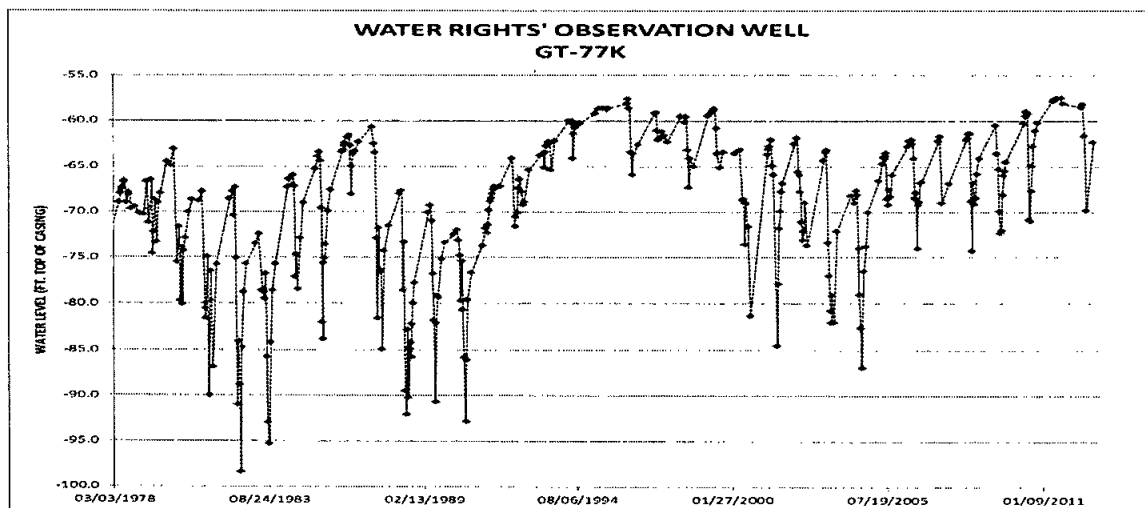
Figure 7- Hydrograph for observation well GT-77K (Water Rights, 2013a)
