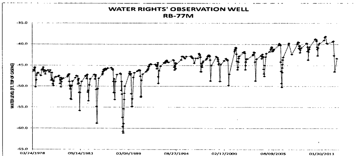
Figure 4- Hydrograph for observation well RB-77M (Water Rights, 2013a)
