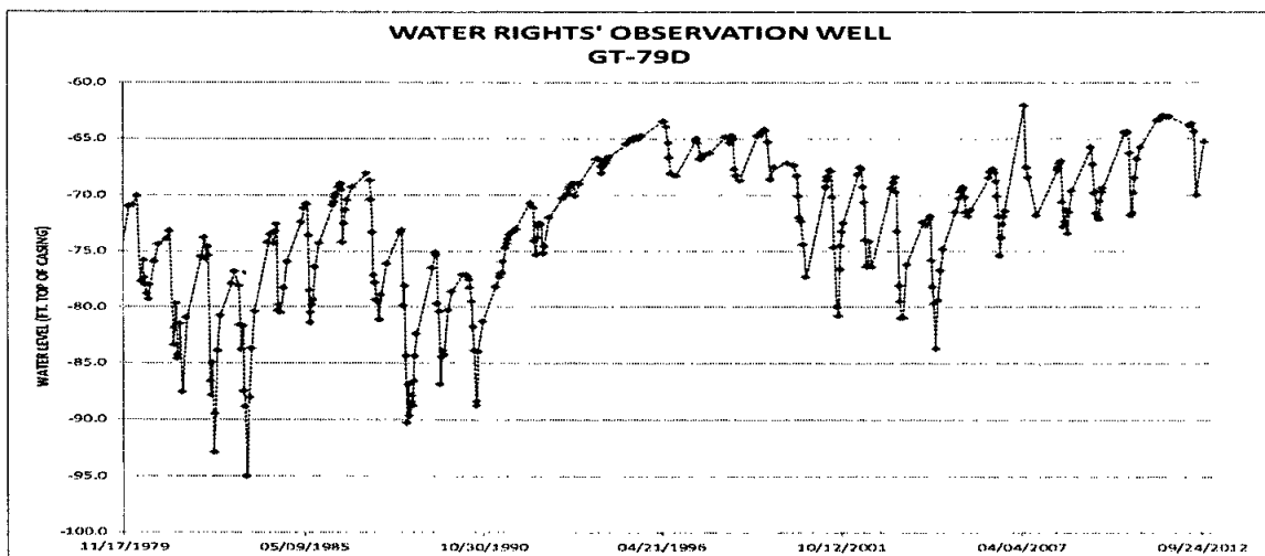
Figure 6- Hydrograph for observation well GT-79D (Water Rights, 2013a)
