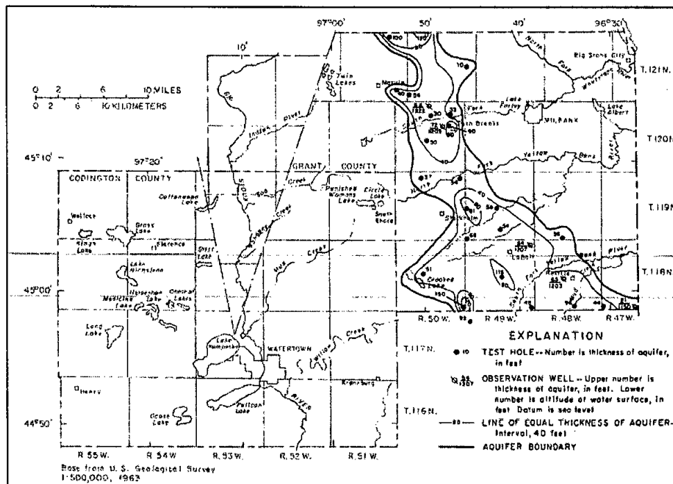
Figure 2- Thickness and extent of the Renvo aquifer in Grant County (modified from Hansen, 1990)
