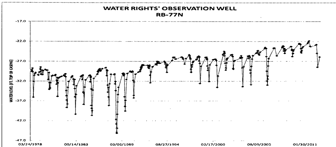
Figure 5- Hydrograph for observation well RB-77N (Water Rights, 2013a)
