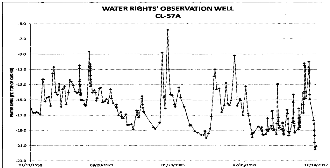
Figure 2. Hydrograph for SD DENR-Water Rights' Observation Well CL-57A completed into the Lower Vermillion-Missouri aquifer less than two miles southwest of the well site proposed by Application No. 7688-3 (Water Rights, 2013a).
