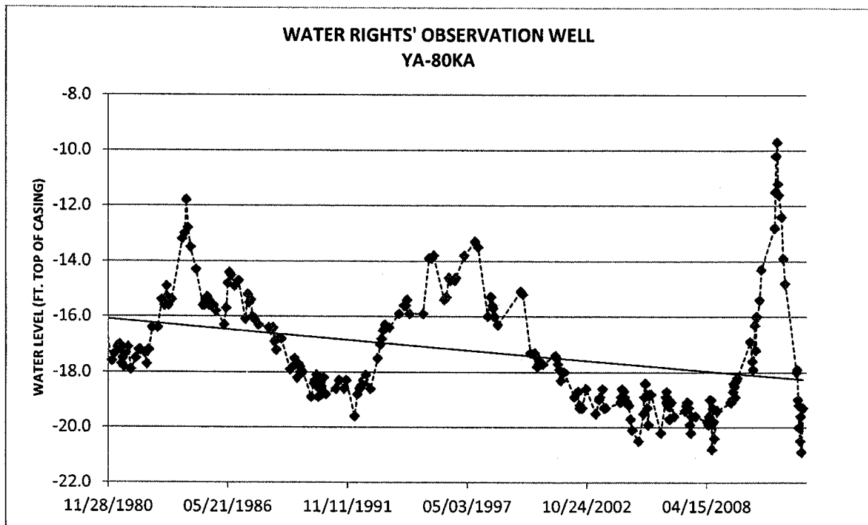
Figure 2. Hydrograph with linear trend line for SD DENR- Water Rights Observation Well YA-80KA completed into the Missouri: Elk Point aquifer less than three miles west of the well site proposed by Application No. 7622-3 (Water Rights, 2013a).
