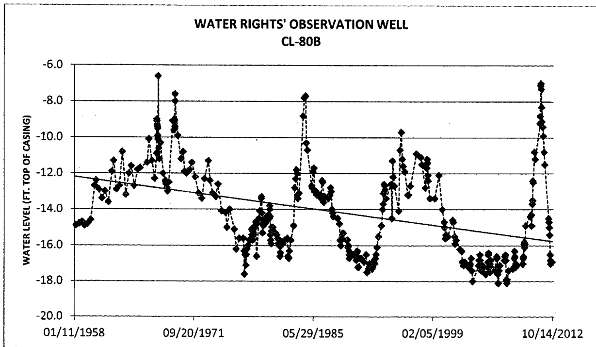
Figure 1. Hydrograph with linear trend line for SD DENR-Water Rights Observation Well CL-80B completed into the Missouri: Elk Point aquifer less than two miles southeast of the well site proposed by Application No. 7621-3 (Water Rights, 2013a).
