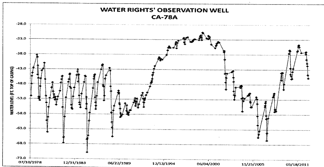
Figure 1- Hydrograph for observation well CA-78A (Water Rights, 2013a)
