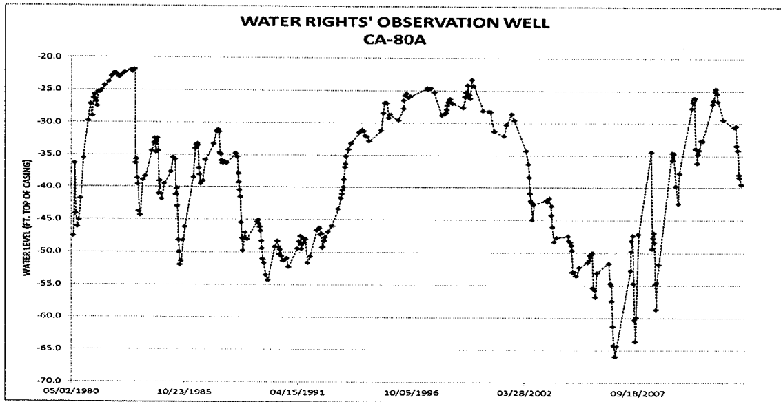
Figure 2- Hydrograph for observation well CA-80A (Water Rights, 2013a)
