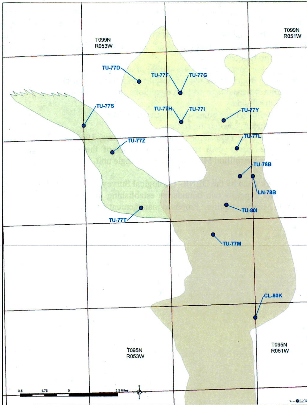
Figure 8. Proposed management units for the Upper Vermillion Missouri aquifer
