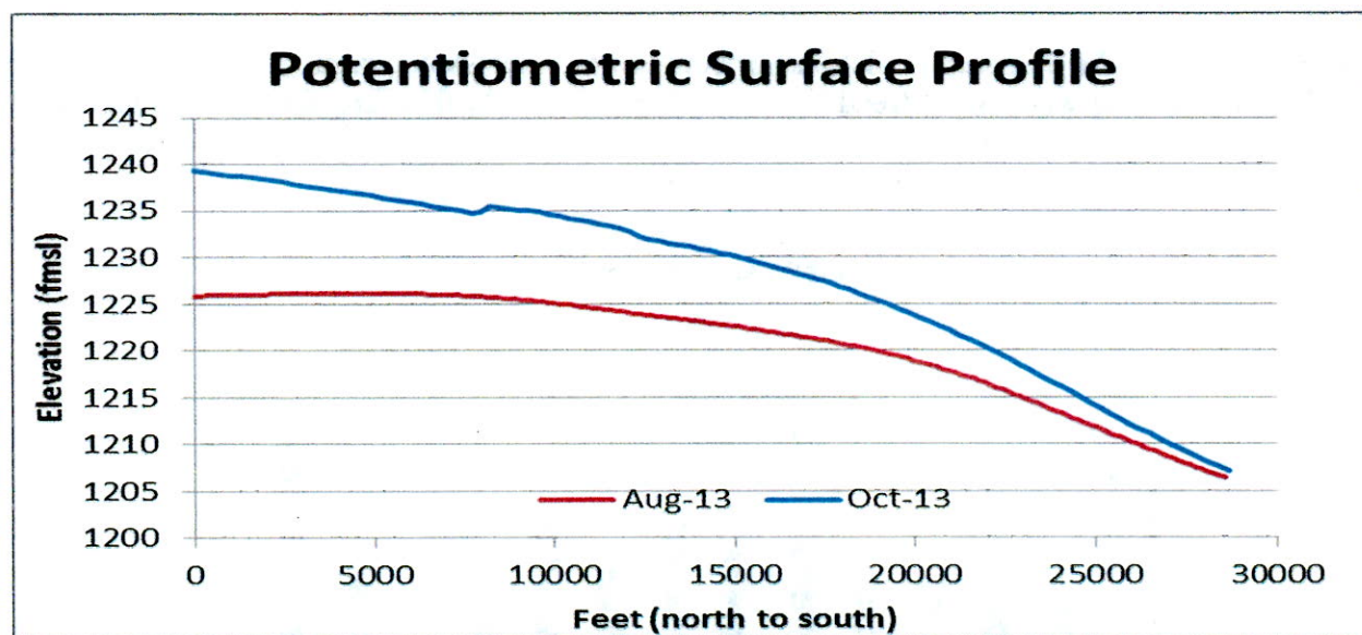
Figure 44. Profile of the potentiometric surface showing stress in North management unit.
