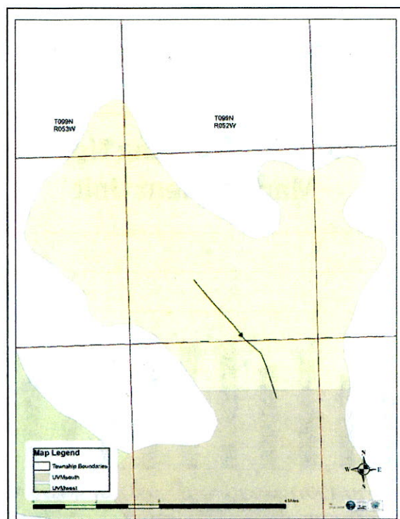
Figure 43. Map showing location of potentiometric surface profile.
