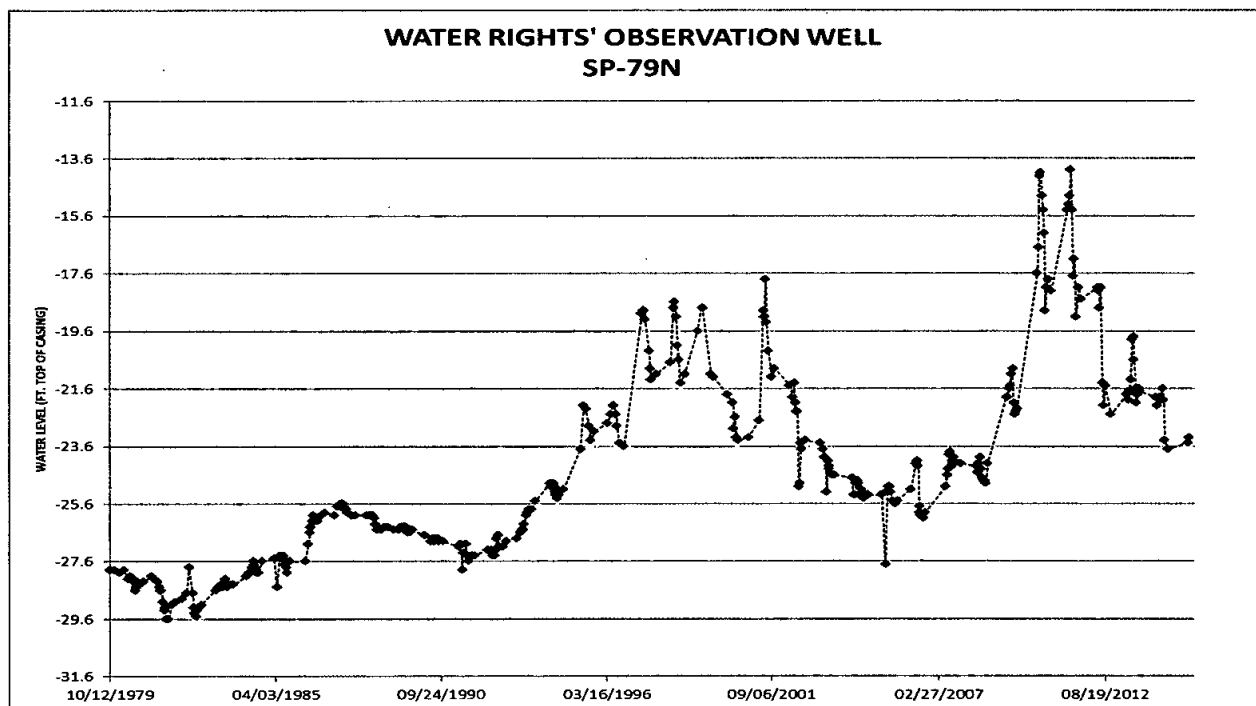
Figure 2. Hydrograph for DENR-Water Rights' observation well completed into the Tulare: Western Spink/Hitchcock aquifer approximately three-fourths of a mile northeast of the wells that supply water for Water Right No. 4794-3.
