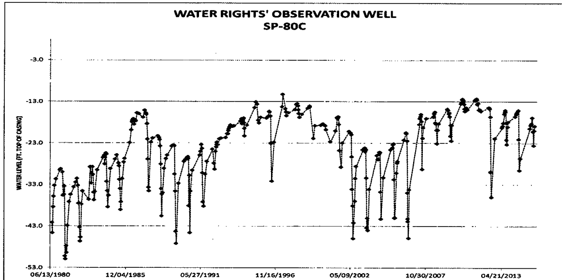
Figure 2. Hydrograph for DENR-Water Rights Program observation well completed into the Tulare: Western Spink/Hitchcock aquifer (Water Rights, 2015a).
