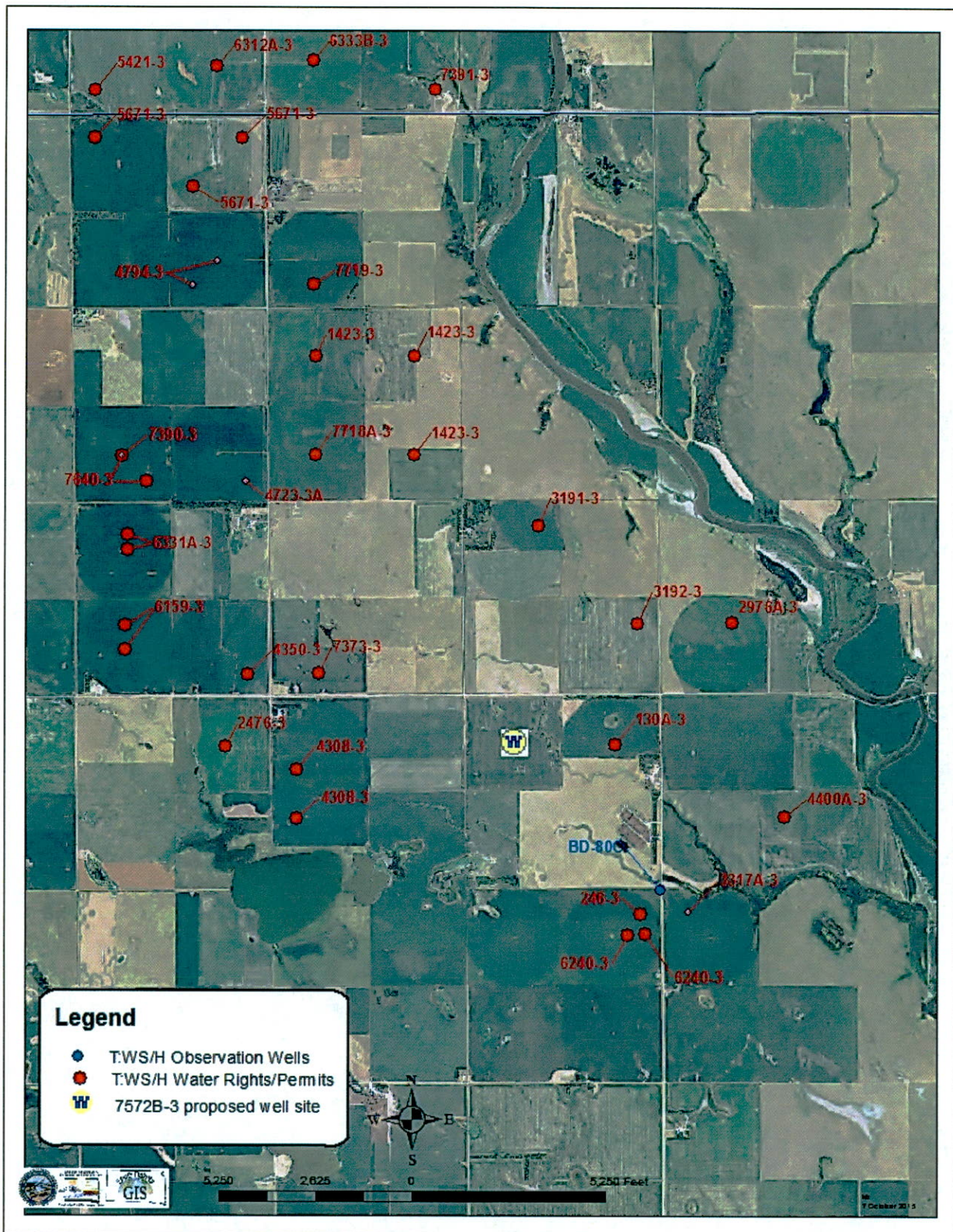
Figure 1. Approximate location of diversion points for Water Rights/Permits appropriating water from the Tulare: Western Spink/Hitchcock aquifer in the vicinity of the well site proposed by Application No. 7572B-3 (Water Rights, 2015b).
