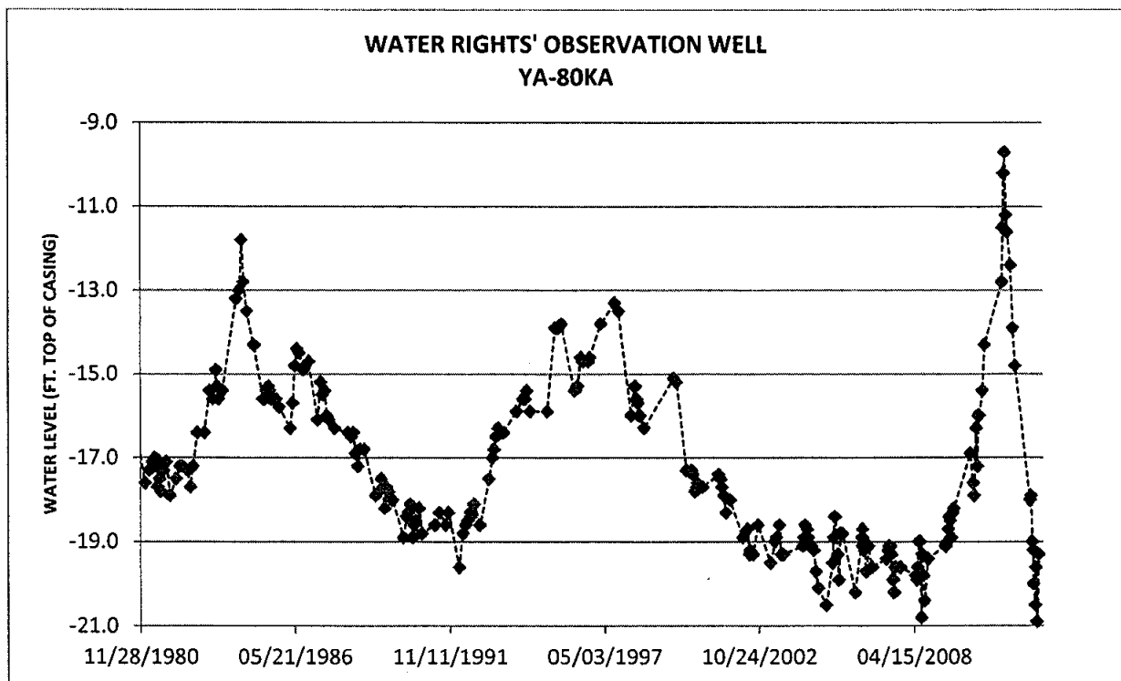
Figure 2. Hydrograph for DENR- Water Rights Observation Well YA-80KA completed into the Missouri: Elk Point aquifer approximately 1.9 miles southeast of the well site proposed by Application No. 7565-3 (Water Rights, 2013a).
