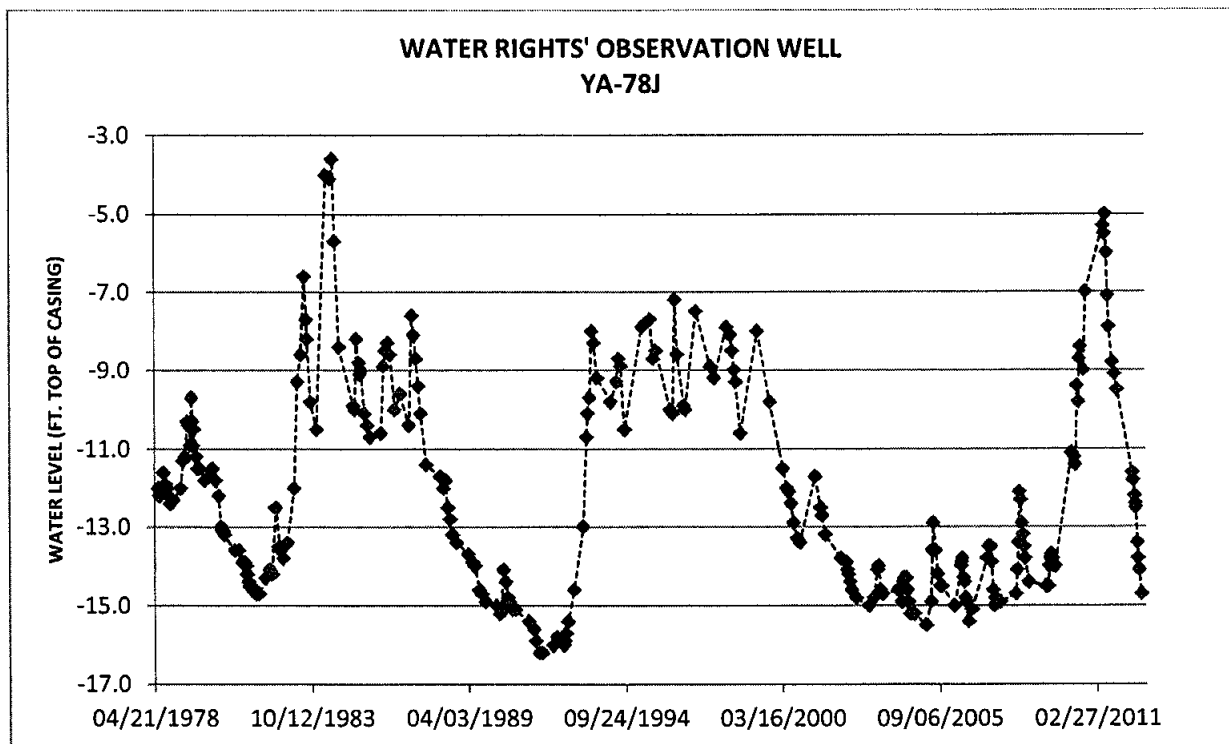
Figure 1. Hydrograph for DENR-Water Rights Observation Well YA-78J completed into the Missouri: Elk Point aquifer approximately 3.6 miles northwest of the well site proposed by Application No. 7565-3 (Water Rights, 2013a).
