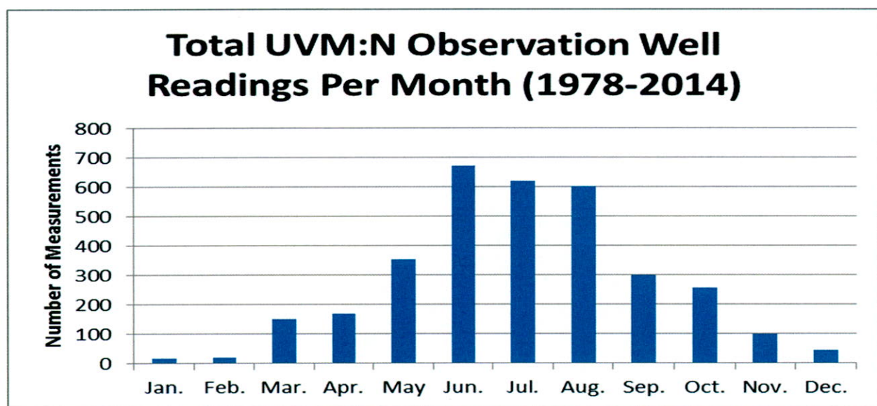
Figure 20. Monthly distribution of water level readings taken from DENR-Observation Wells completed into the Upper Vermillion Missouri: North aquifer for 1978-2014 (Water Rights, 2015a).
