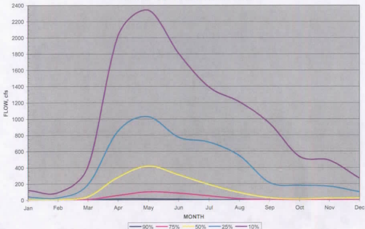
James River Gage at Ashton, SD 1945 - 2010
