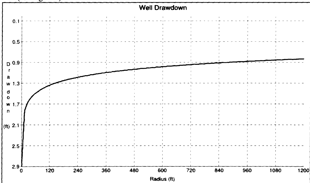
Figure 1. Drawdown versus distance graph based on the Theis Solution, for a production well completed into the Big Sioux: Brookings aquifer where: T=97,240 GPD/ft, S=0.004 , t=365 days, Q=95 gpm
