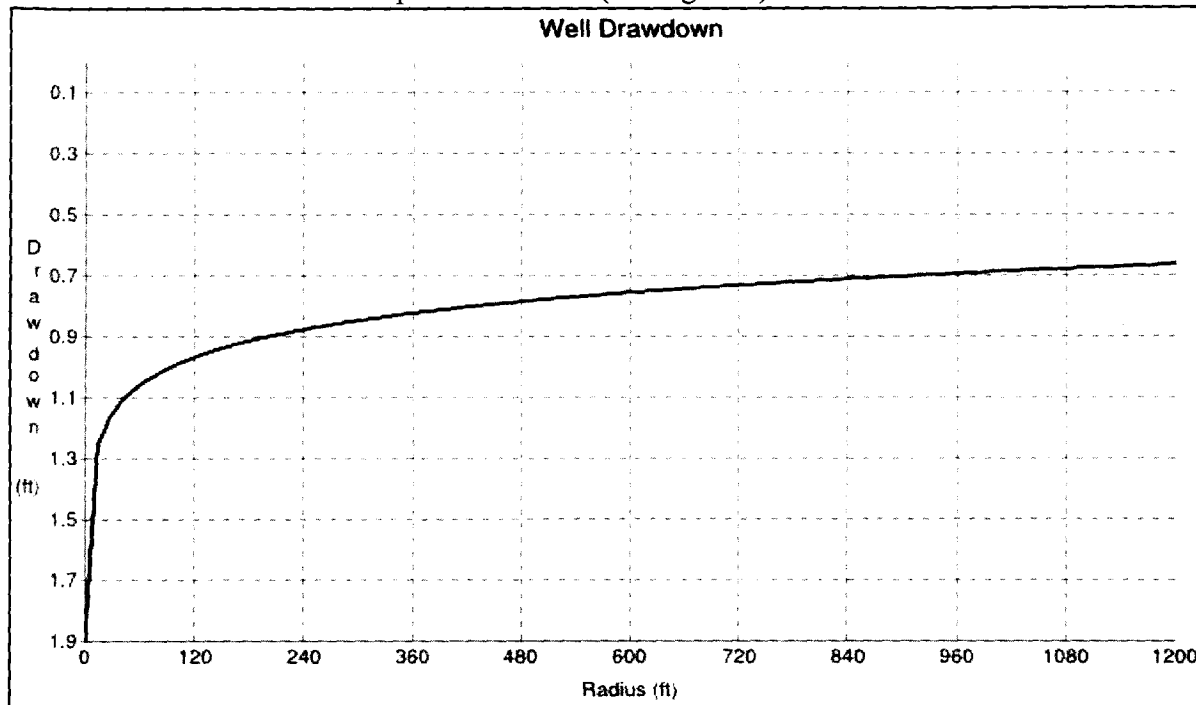
Figure 2. Drawdown versus distance graph based on the Theis Solution, for a production well completed into the Prairie Coteau aquifer where: T=166,380 GPD/ft, S=0.0005 , t=365 days, Q=95 gpm
