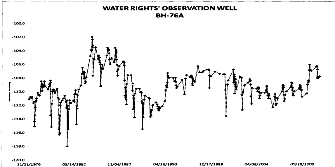
Figure 2. Hydrograph of DENR-Water Rights' Observation Well BH-76A which is located approximately 1.8 miles southwest of the well site proposed by Application No. 7331-3.
