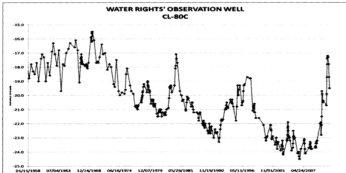
Figure 2. Hydrograph of DENR-Water Rights' Observation Well CL-80C which is located approximately nine-tenths of a mile south-southwest of the well Application No. 7300-3 proposes to use.
