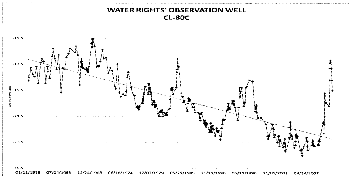
Figure 5. Hydrograph of Water Rights' Observation Well CL-80C, with linear trend line.
