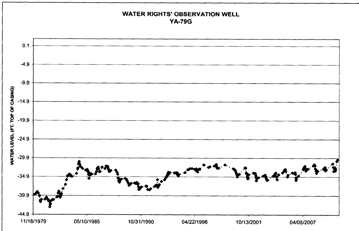
Figure 2. Hydrograph for Water Rights Observation Well YA-79G, completed into the Lower James Missouri:Scotland Aquifer within one mile of 7220-3
