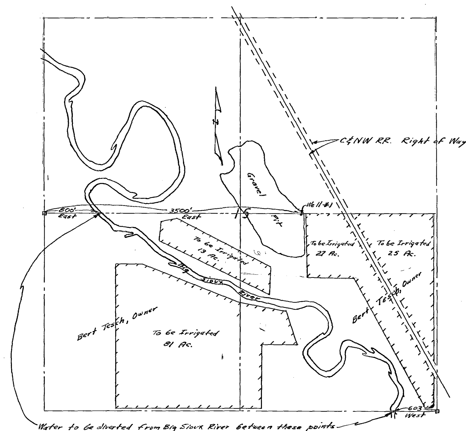
SECTION 15, T 116 N, R 52 W of the Fifth P.M. 1" = 660' □ Indicates Corners Used for Measuring
