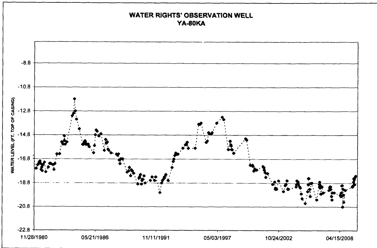
Figure 1. Hydrograph for Water Rights Observation Well YA-80KA, completed into the Missouri Elk Point Aquifer within one mile of 7199-3.
