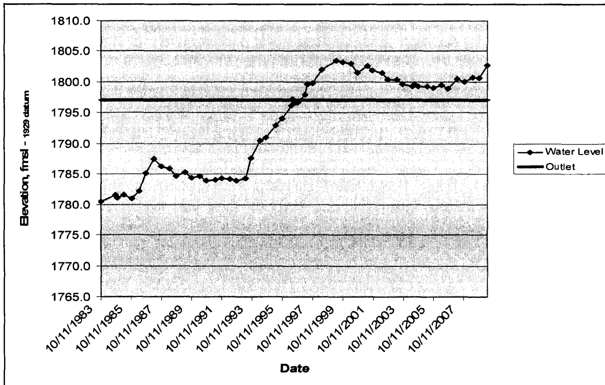
Figure1. Measured water levels on Waubay Lake, 1983 – Present.
