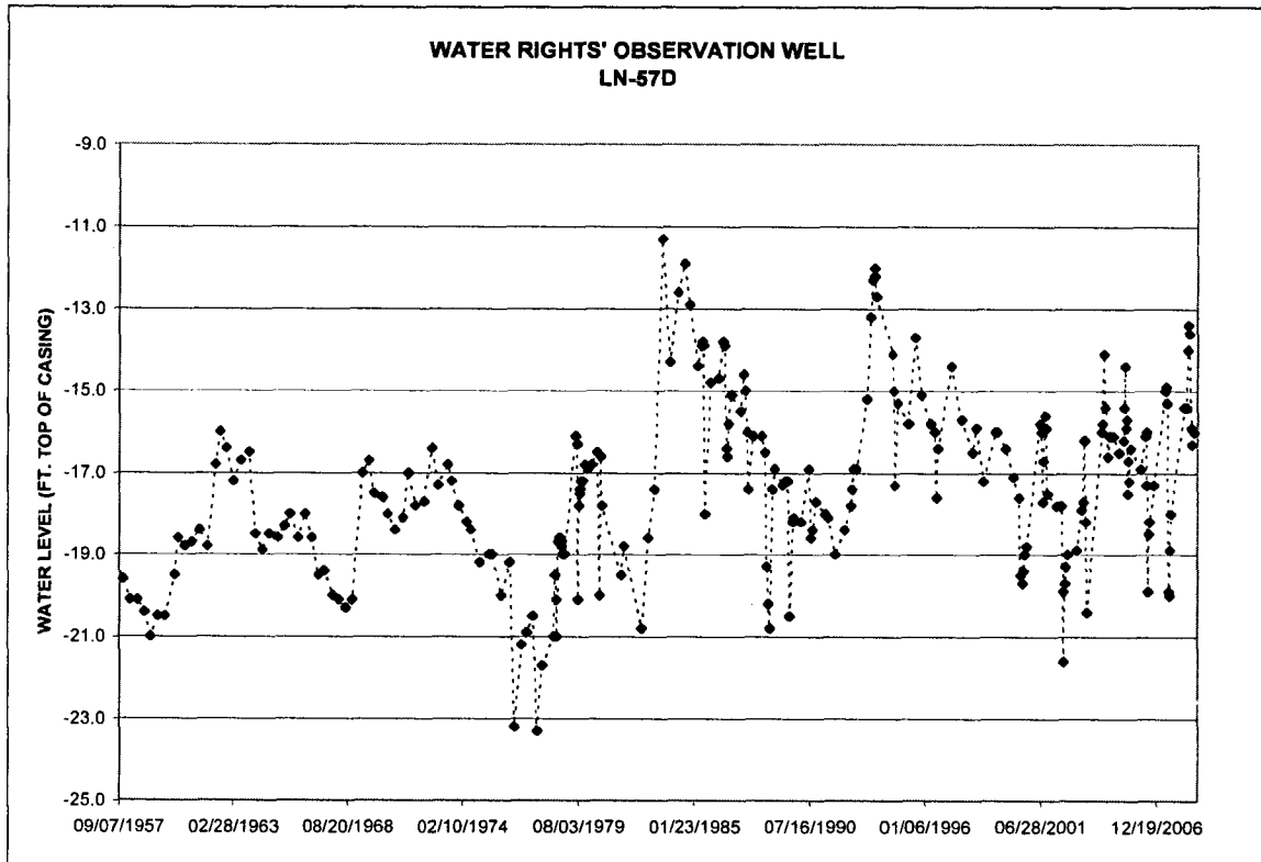
Figure 1. Hydrograph for Water Rights Observation Well LN-57D, completed into the Big Sioux South Aquifer within one mile of 7108-3
