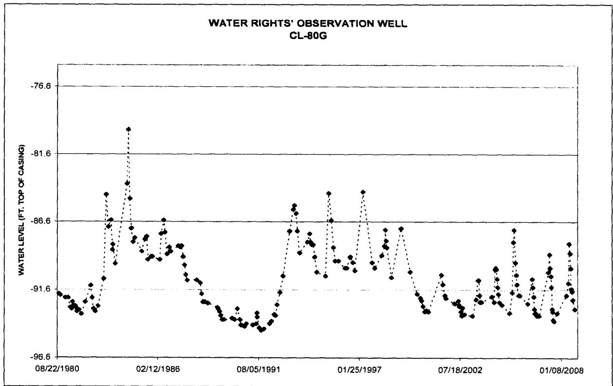
Figure 2. Hydrograph for Water Rights Observation Well CL-80G, completed into the Lower Vermillion Missouri Aquifer within two miles of 7082-3
