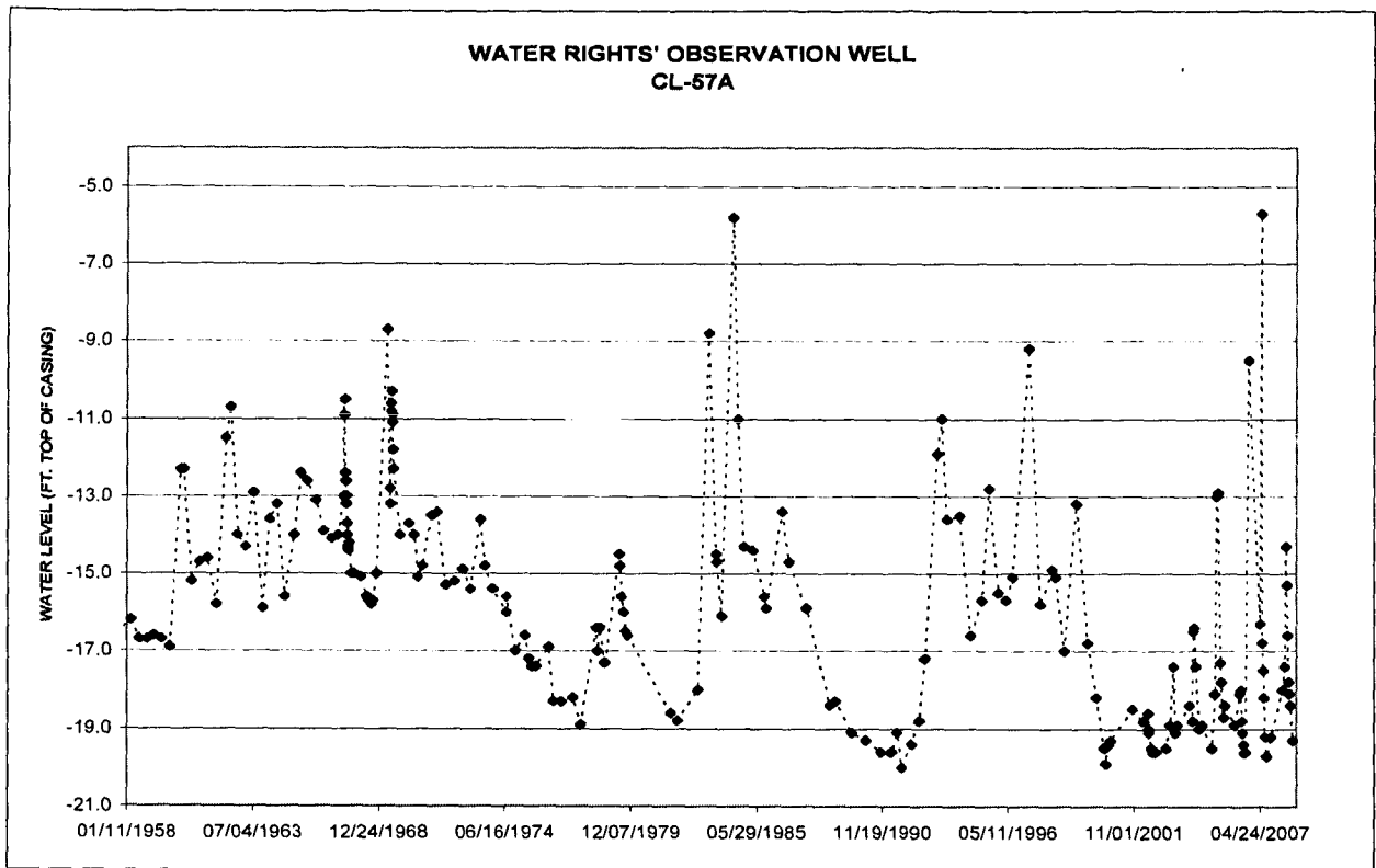
Figure 1. Hydrograph for Water Rights Observation Well CL-57A, completed into the Lower Vermillion Missouri Aquifer within two miles of 7082-3
