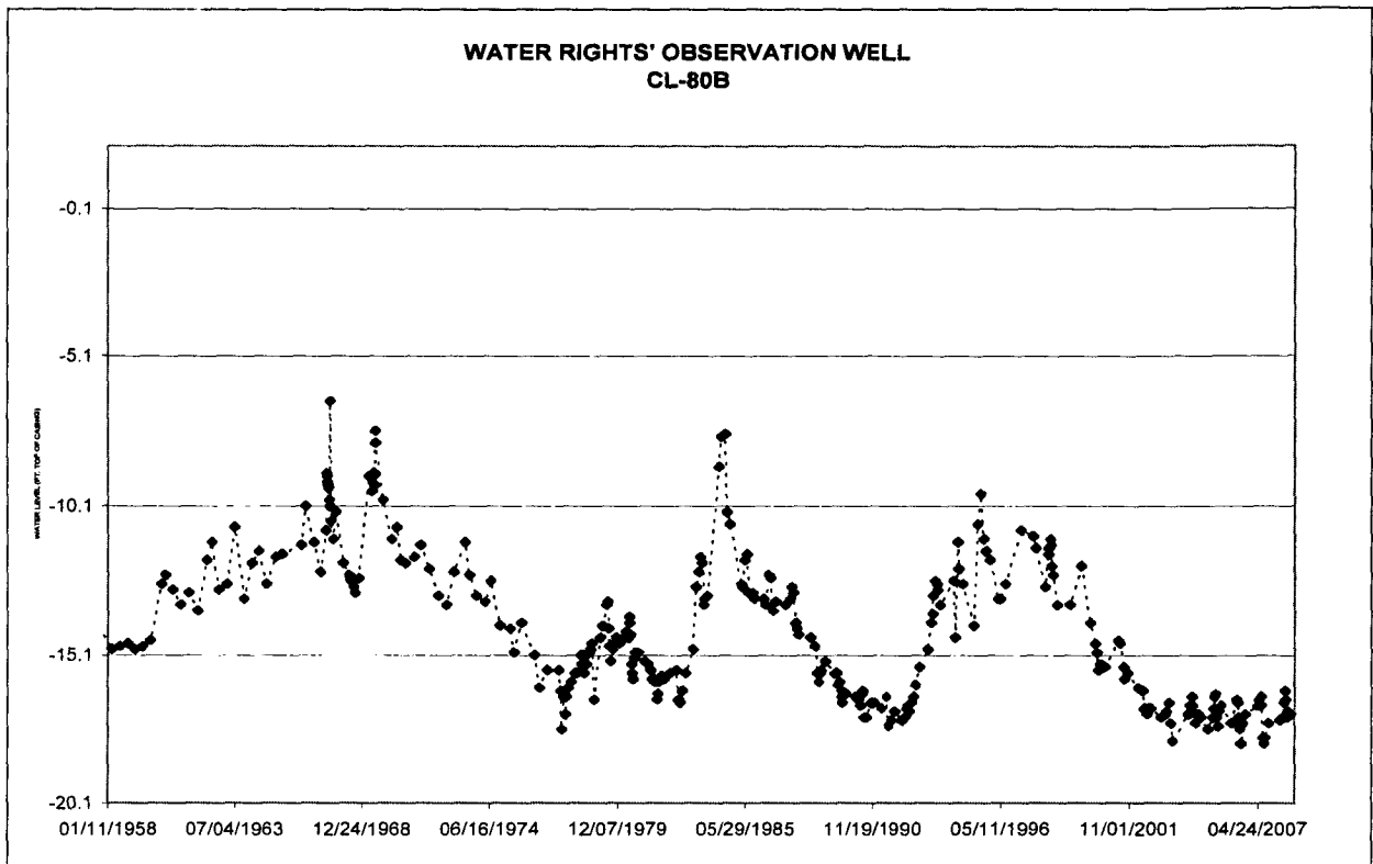
Figure 1. Hydrograph for Water Rights Observation Well CL-80B, completed into the Elk Point management unit of the Missouri Aquifer within four miles of 7075-3
