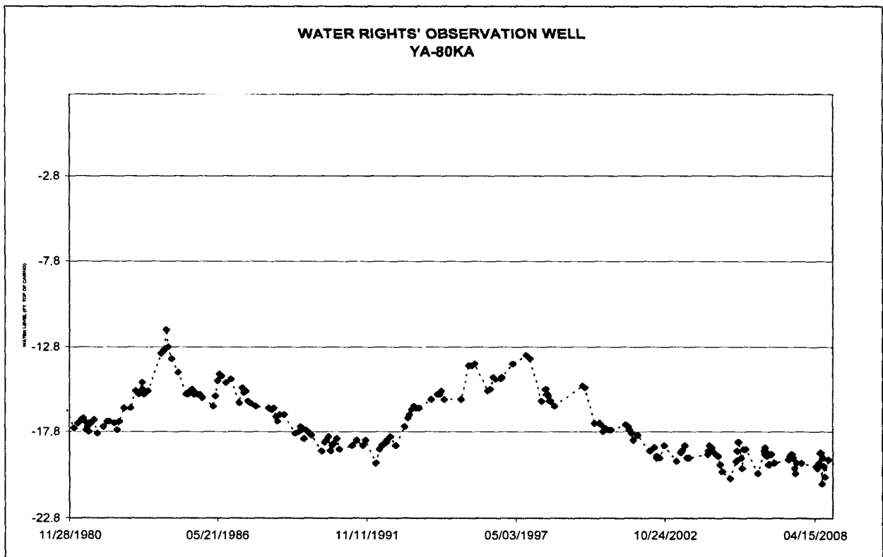
Figure 2. Hydrograph for Water Rights Observation Well YA-80KA, completed into the Elk Point management unit of the Missouri Aquifer within four miles of 7075-3
